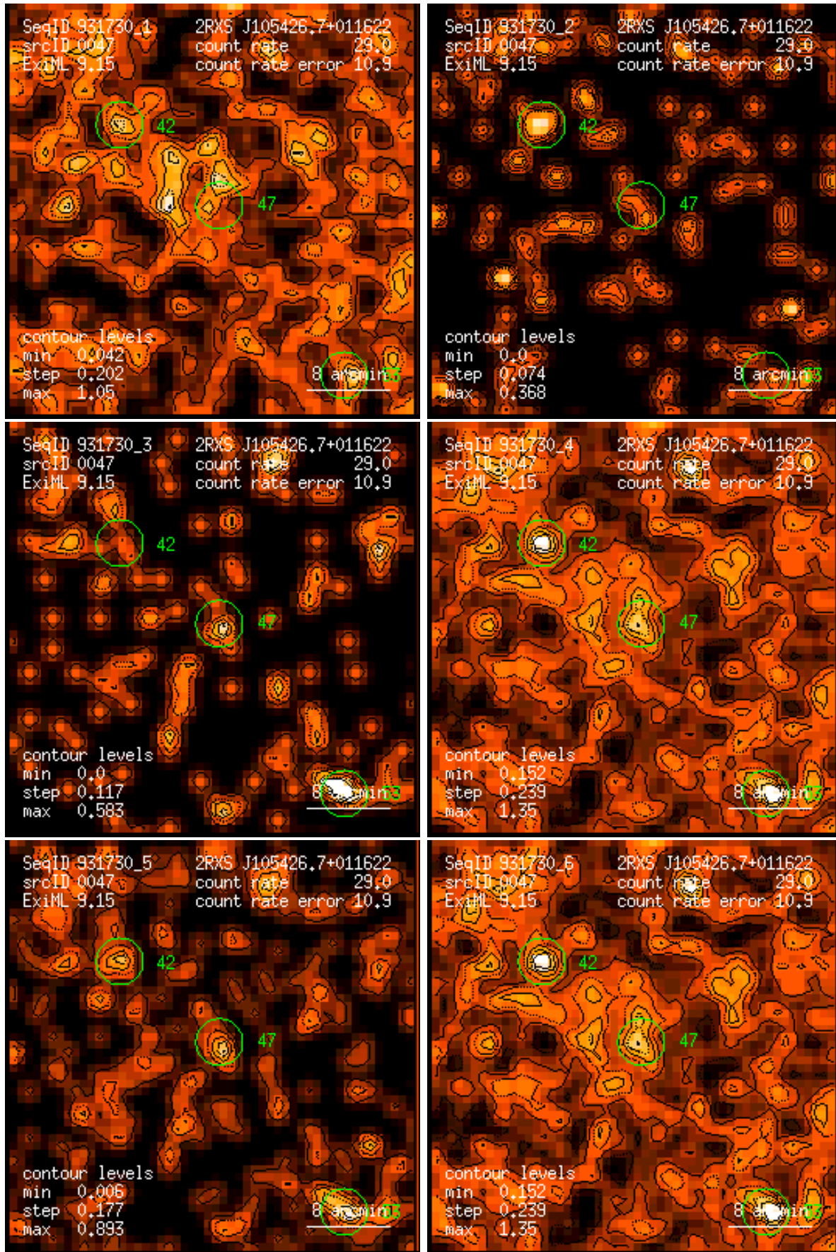
Figure 47: RASS 931730: detection 0047: band rate images, Gaussian filter: (1) PSPC channels 11 – 41, (2) 52 – 90, (3) 91 – 201, (4) 11 – 235, (5) 52 – 201, (6) 11 – 201. Broad band rates in counts/ks. Band rate contour levels in counts/ks/arcmin 2 .
