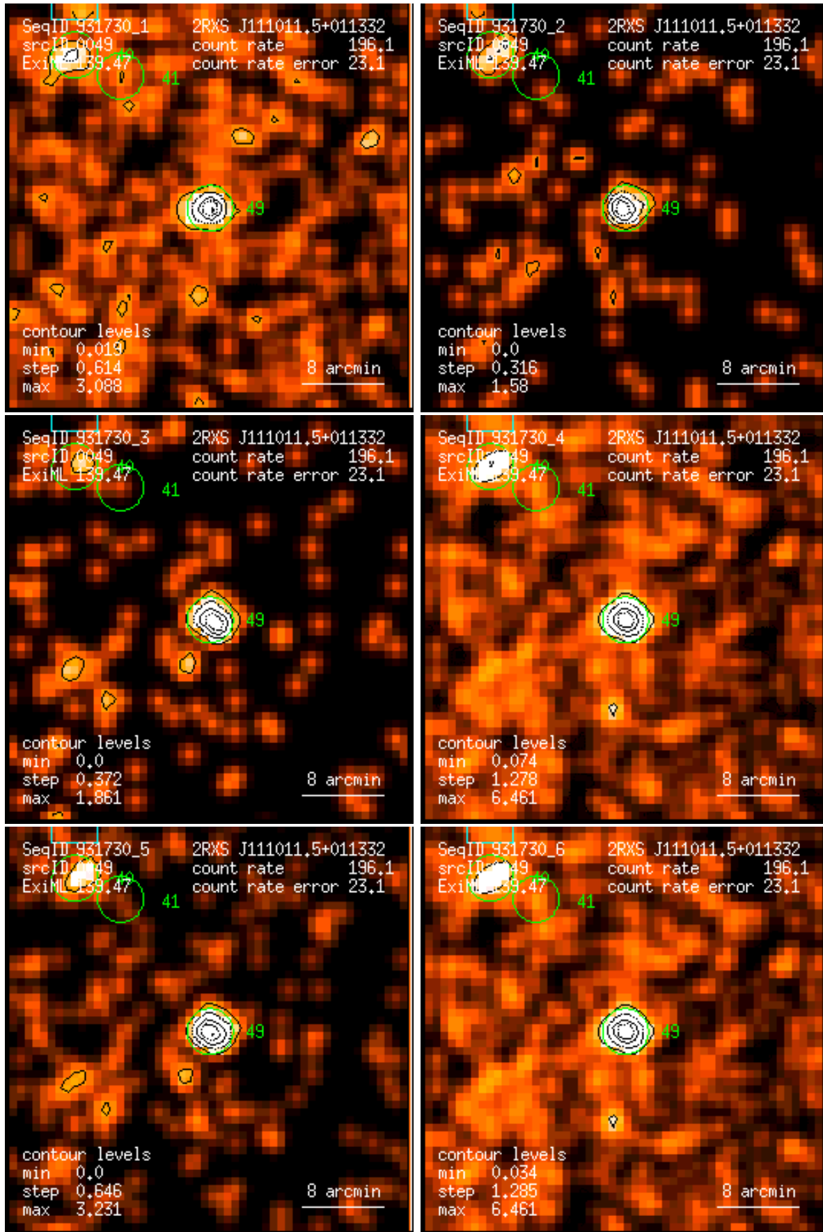
Figure 49: RASS 931730: detection 0049: band rate images, Gaussian filter: (1) PSPC channels 11 – 41, (2) 52 – 90, (3) 91 – 201, (4) 11 – 235, (5) 52 – 201, (6) 11 – 201. Broad band rates in counts/ks. Band rate contour levels in counts/ks/arcmin 2 .
