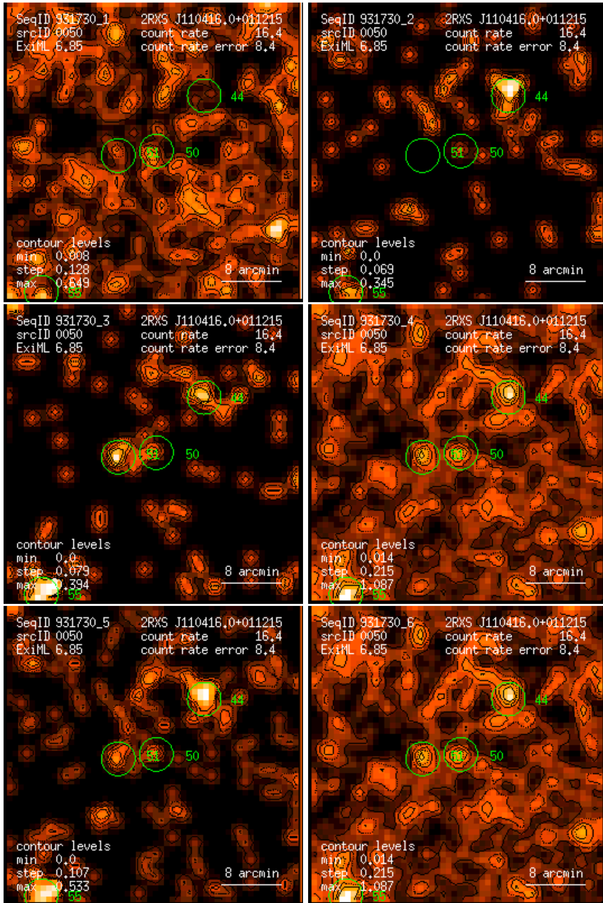
Figure 50: RASS 931730: detection 0050: band rate images, Gaussian filter: (1) PSPC channels 11 – 41, (2) 52 – 90, (3) 91 – 201, (4) 11 – 235, (5) 52 – 201, (6) 11 – 201. Broad band rates in counts/ks. Band rate contour levels in counts/ks/arcmin 2 .
