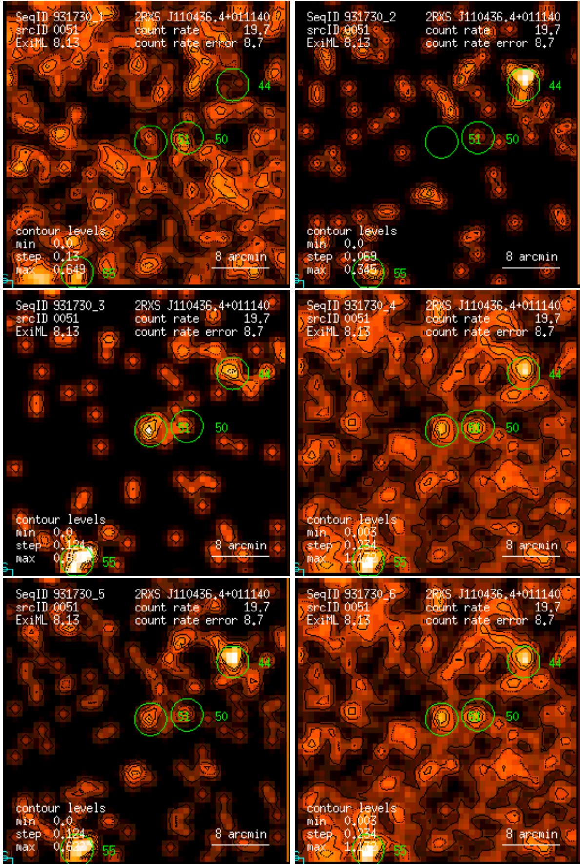
Figure 51: RASS 931730: detection 0051: band rate images, Gaussian filter: (1) PSPC channels 11 – 41, (2) 52 – 90, (3) 91 – 201, (4) 11 – 235, (5) 52 – 201, (6) 11 – 201. Broad band rates in counts/ks. Band rate contour levels in counts/ks/arcmin 2 .
