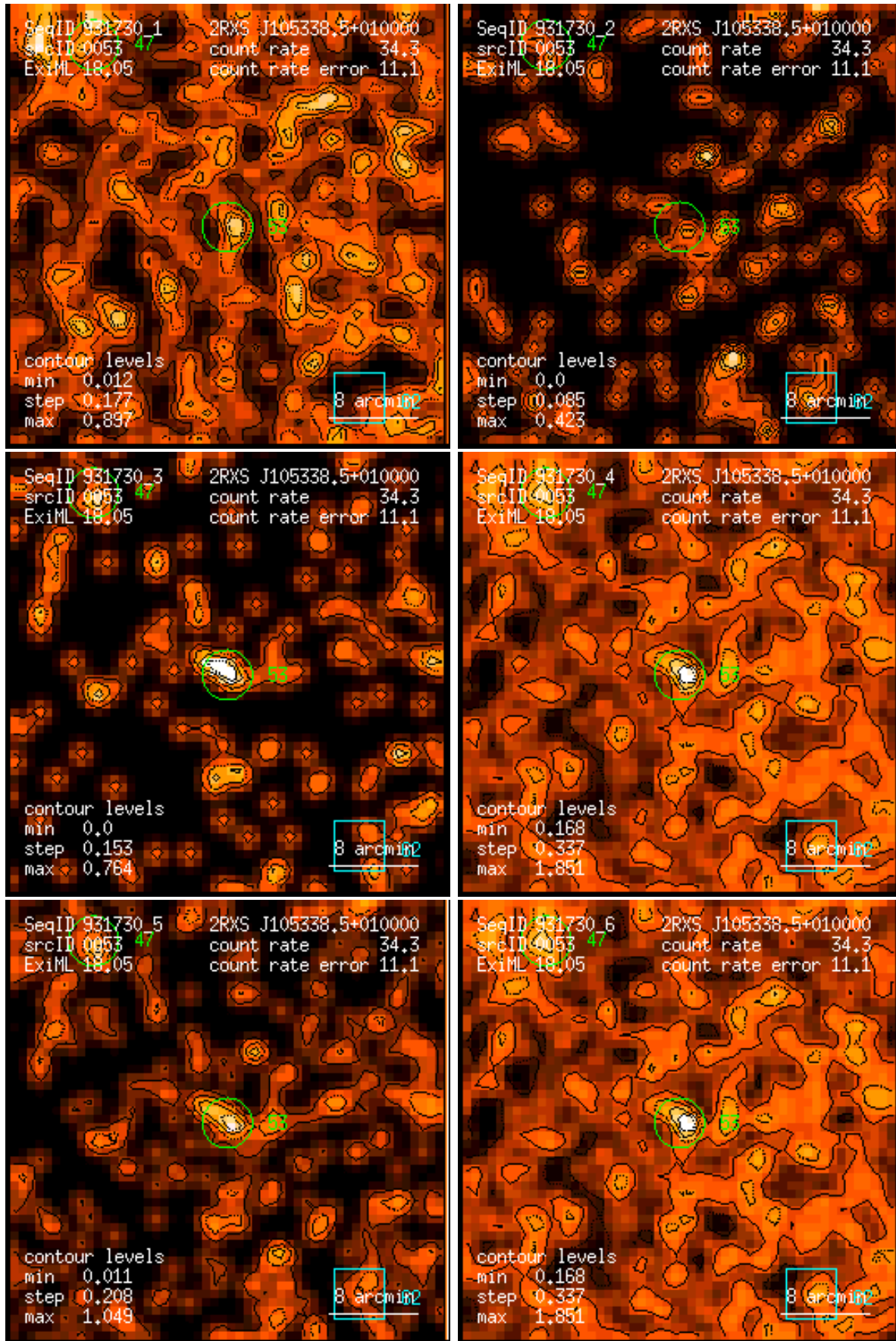
Figure 53: RASS 931730: detection 0053: band rate images, Gaussian filter: (1) PSPC channels 11 – 41, (2) 52 – 90, (3) 91 – 201, (4) 11 – 235, (5) 52 – 201, (6) 11 – 201. Broad band rates in counts/ks. Band rate contour levels in counts/ks/arcmin 2 .
