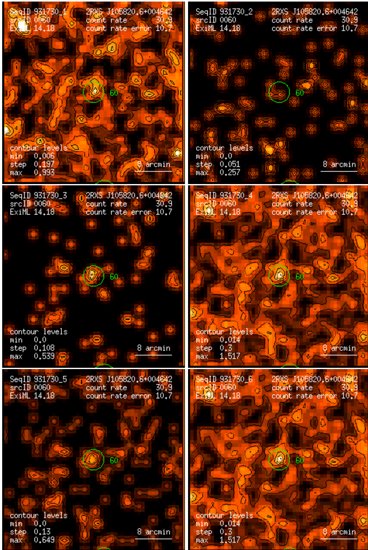
Figure 60: RASS 931730: detection 0060: band rate images, Gaussian filter: (1) PSPC channels 11 – 41, (2) 52 – 90, (3) 91 – 201, (4) 11 – 235, (5) 52 – 201, (6) 11 – 201. Broad band rates in counts/ks. Band rate contour levels in counts/ks/arcmin 2 .
