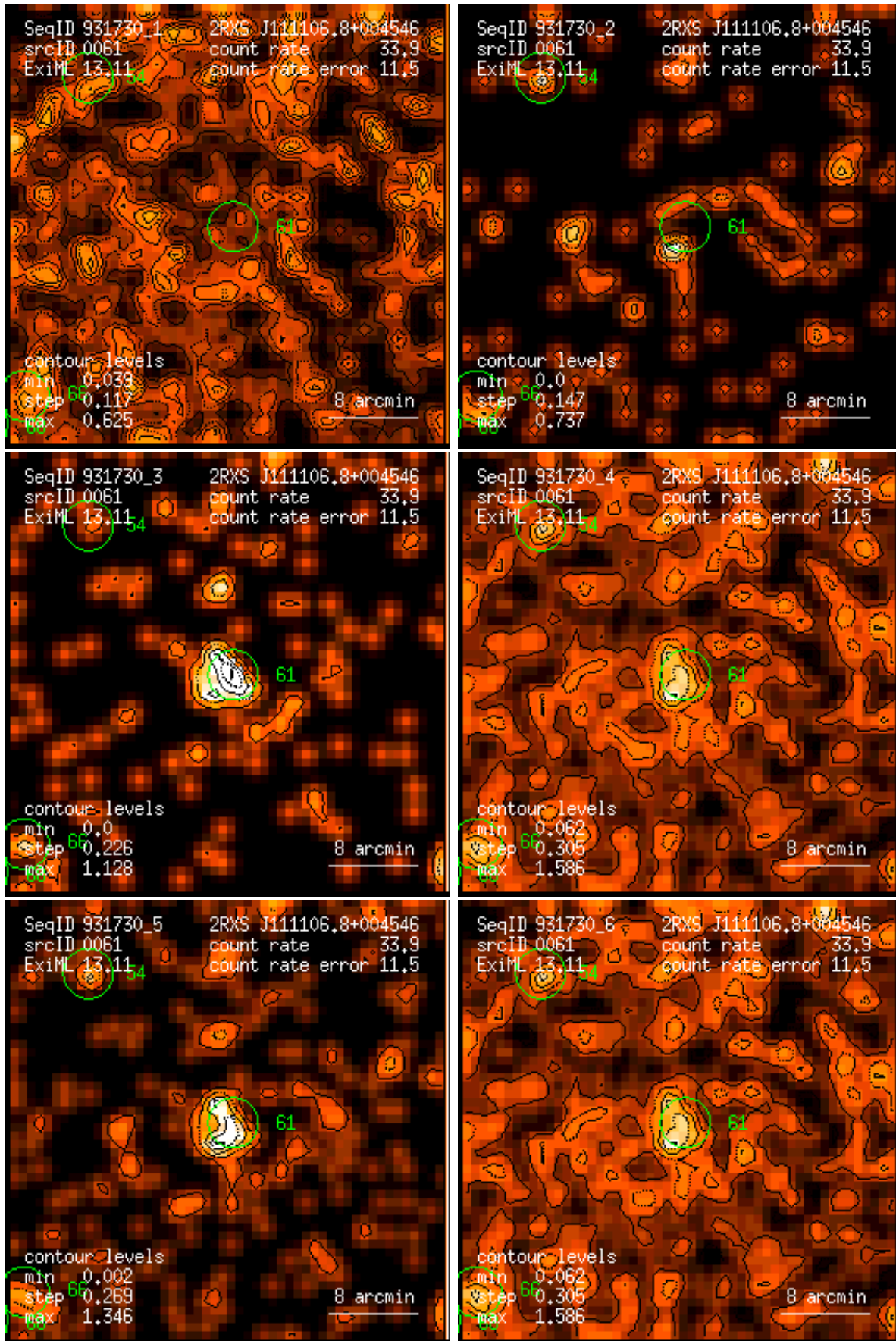
Figure 61: RASS 931730: detection 0061: band rate images, Gaussian filter: (1) PSPC channels 11 – 41, (2) 52 – 90, (3) 91 – 201, (4) 11 – 235, (5) 52 – 201, (6) 11 – 201. Broad band rates in counts/ks. Band rate contour levels in counts/ks/arcmin 2 .
