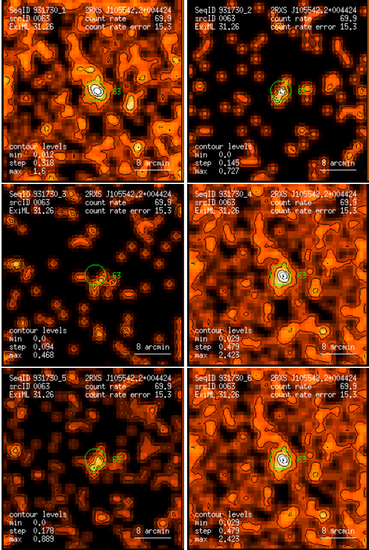
Figure 63: RASS 931730: detection 0063: band rate images, Gaussian filter: (1) PSPC channels 11 – 41, (2) 52 – 90, (3) 91 – 201, (4) 11 – 235, (5) 52 – 201, (6) 11 – 201. Broad band rates in counts/ks. Band rate contour levels in counts/ks/arcmin 2 .
