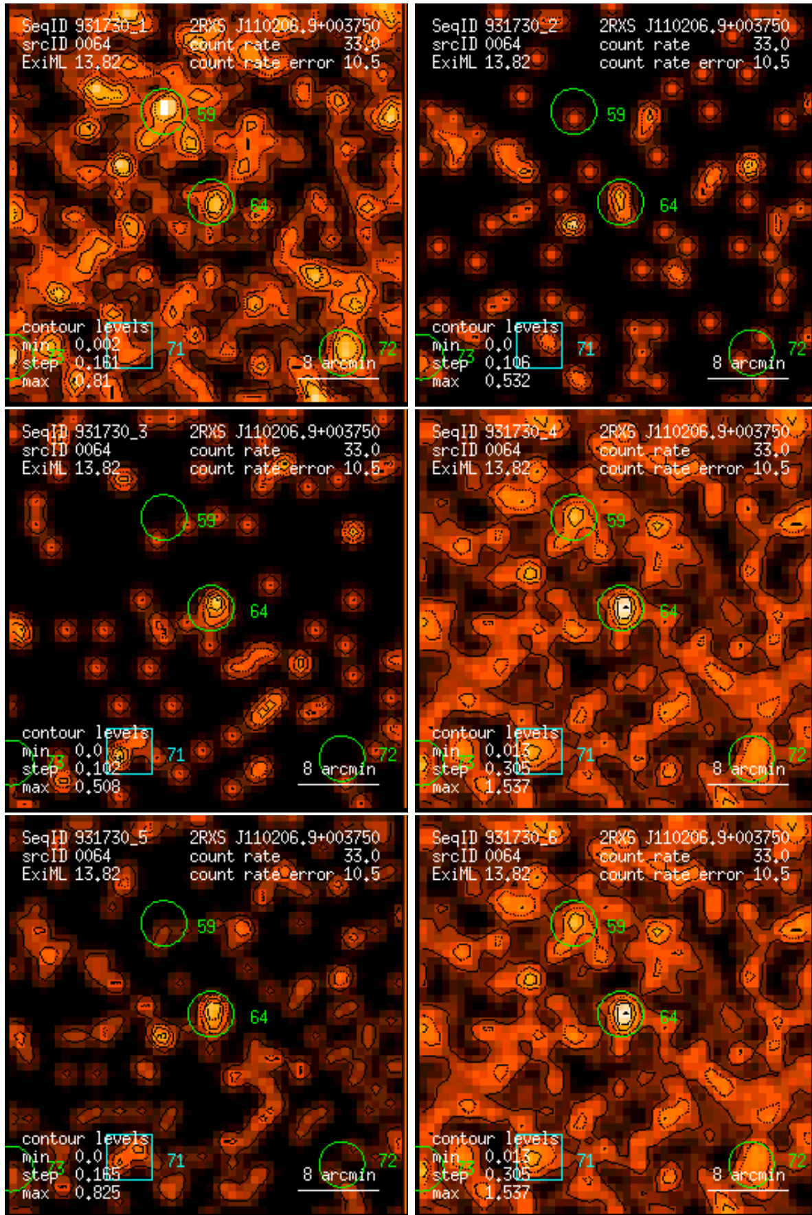
Figure 64: RASS 931730: detection 0064: band rate images, Gaussian filter: (1) PSPC channels 11 – 41, (2) 52 – 90, (3) 91 – 201, (4) 11 – 235, (5) 52 – 201, (6) 11 – 201. Broad band rates in counts/ks. Band rate contour levels in counts/ks/arcmin 2 .
