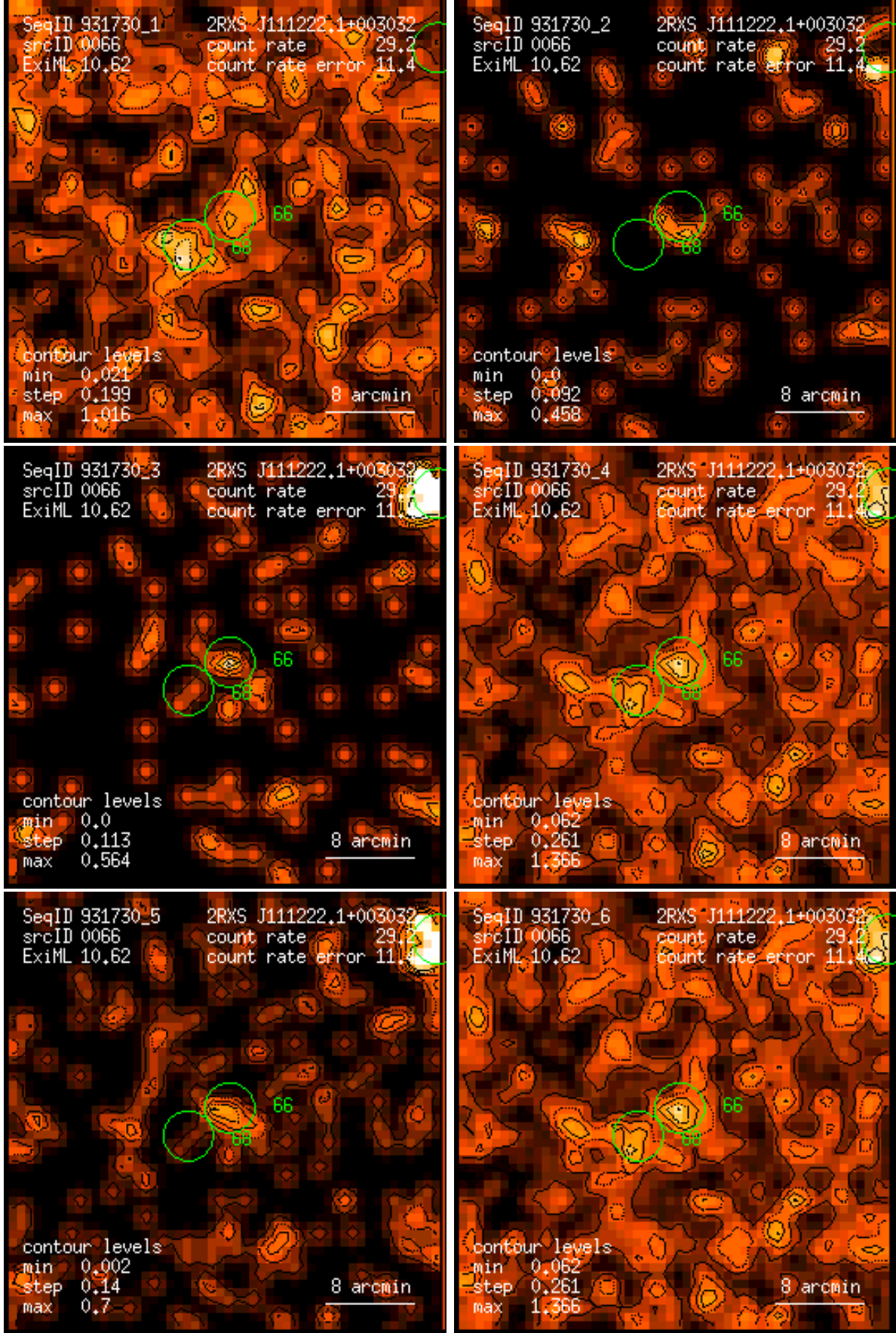
Figure 66: RASS 931730: detection 0066: band rate images, Gaussian filter: (1) PSPC channels 11 – 41, (2) 52 – 90, (3) 91 – 201, (4) 11 – 235, (5) 52 – 201, (6) 11 – 201. Broad band rates in counts/ks. Band rate contour levels in counts/ks/arcmin 2 .
