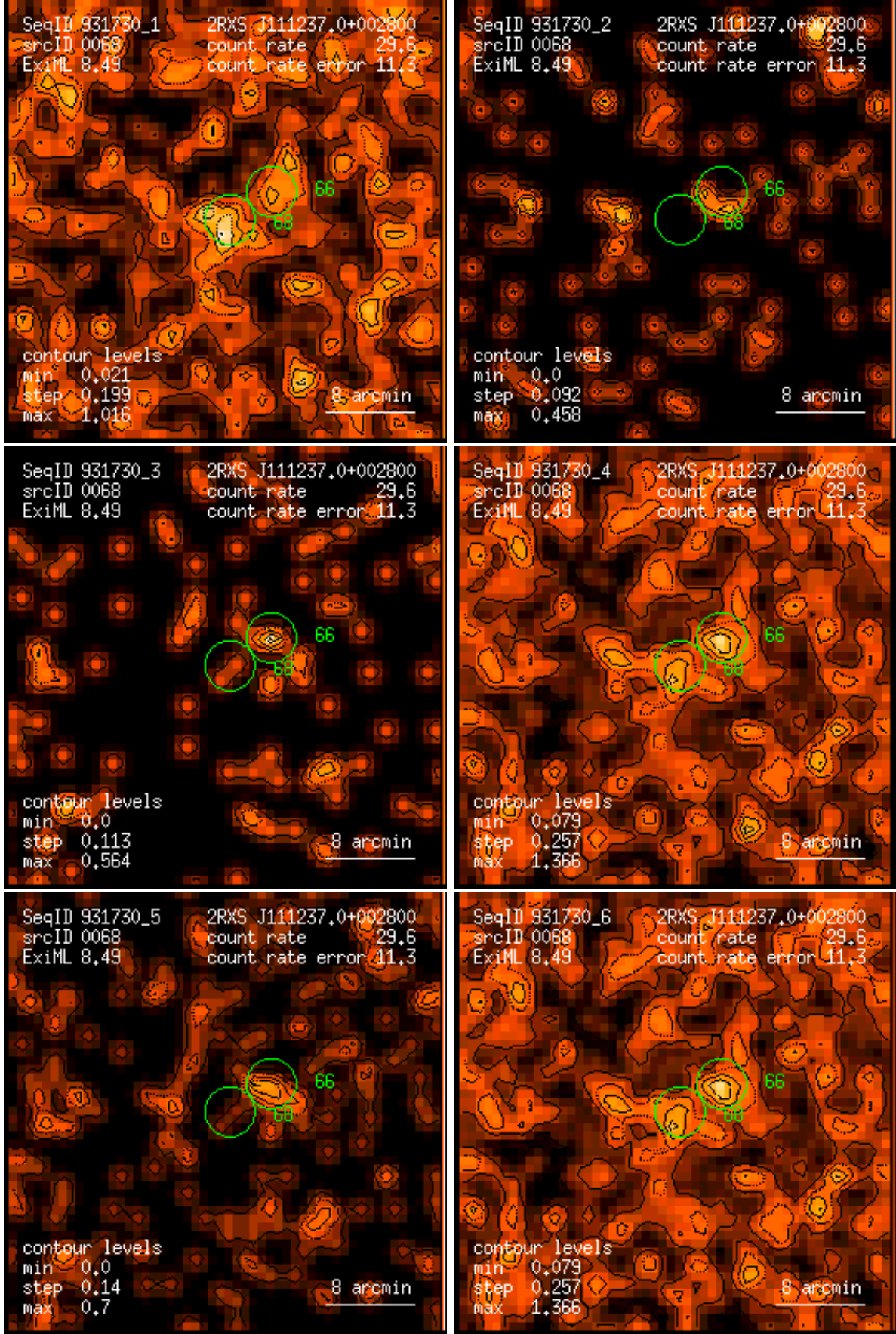
Figure 68: RASS 931730: detection 0068: band rate images, Gaussian filter: (1) PSPC channels 11 – 41, (2) 52 – 90, (3) 91 – 201, (4) 11 – 235, (5) 52 – 201, (6) 11 – 201. Broad band rates in counts/ks. Band rate contour levels in counts/ks/arcmin 2 .
