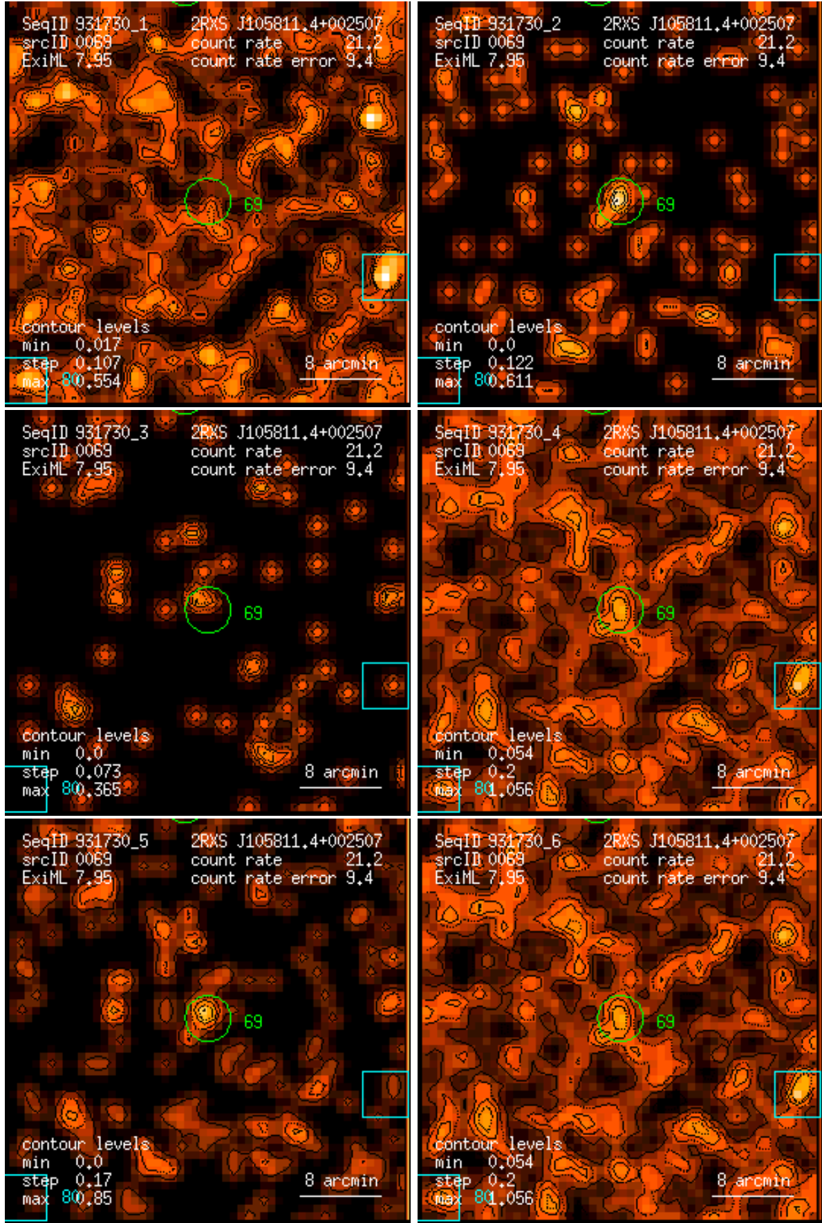
Figure 69: RASS 931730: detection 0069: band rate images, Gaussian filter: (1) PSPC channels 11 – 41, (2) 52 – 90, (3) 91 – 201, (4) 11 – 235, (5) 52 – 201, (6) 11 – 201. Broad band rates in counts/ks. Band rate contour levels in counts/ks/arcmin 2 .
