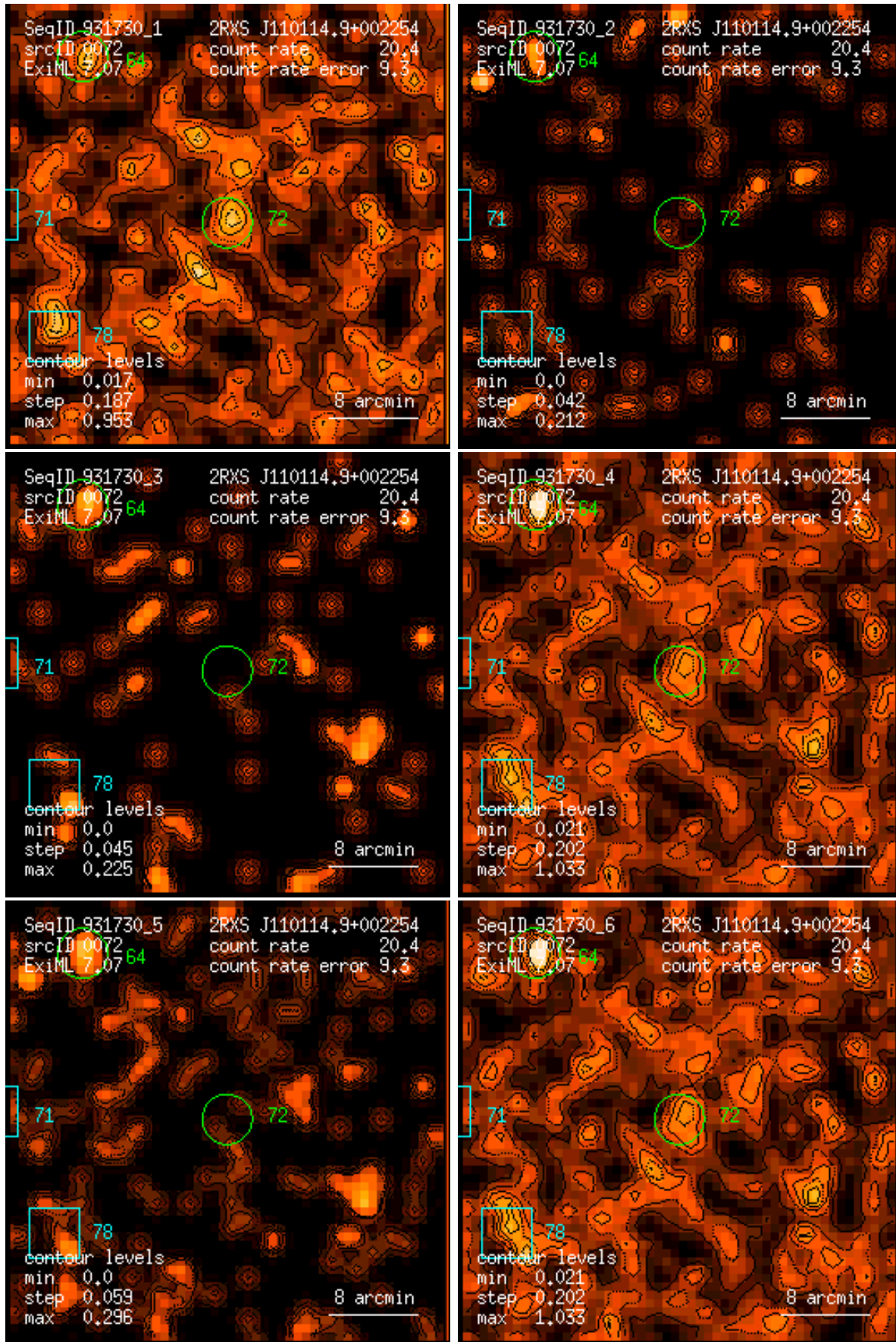
Figure 72: RASS 931730: detection 0072: band rate images, Gaussian filter: (1) PSPC channels 11 – 41, (2) 52 – 90, (3) 91 – 201, (4) 11 – 235, (5) 52 – 201, (6) 11 – 201. Broad band rates in counts/ks. Band rate contour levels in counts/ks/arcmin 2 .
