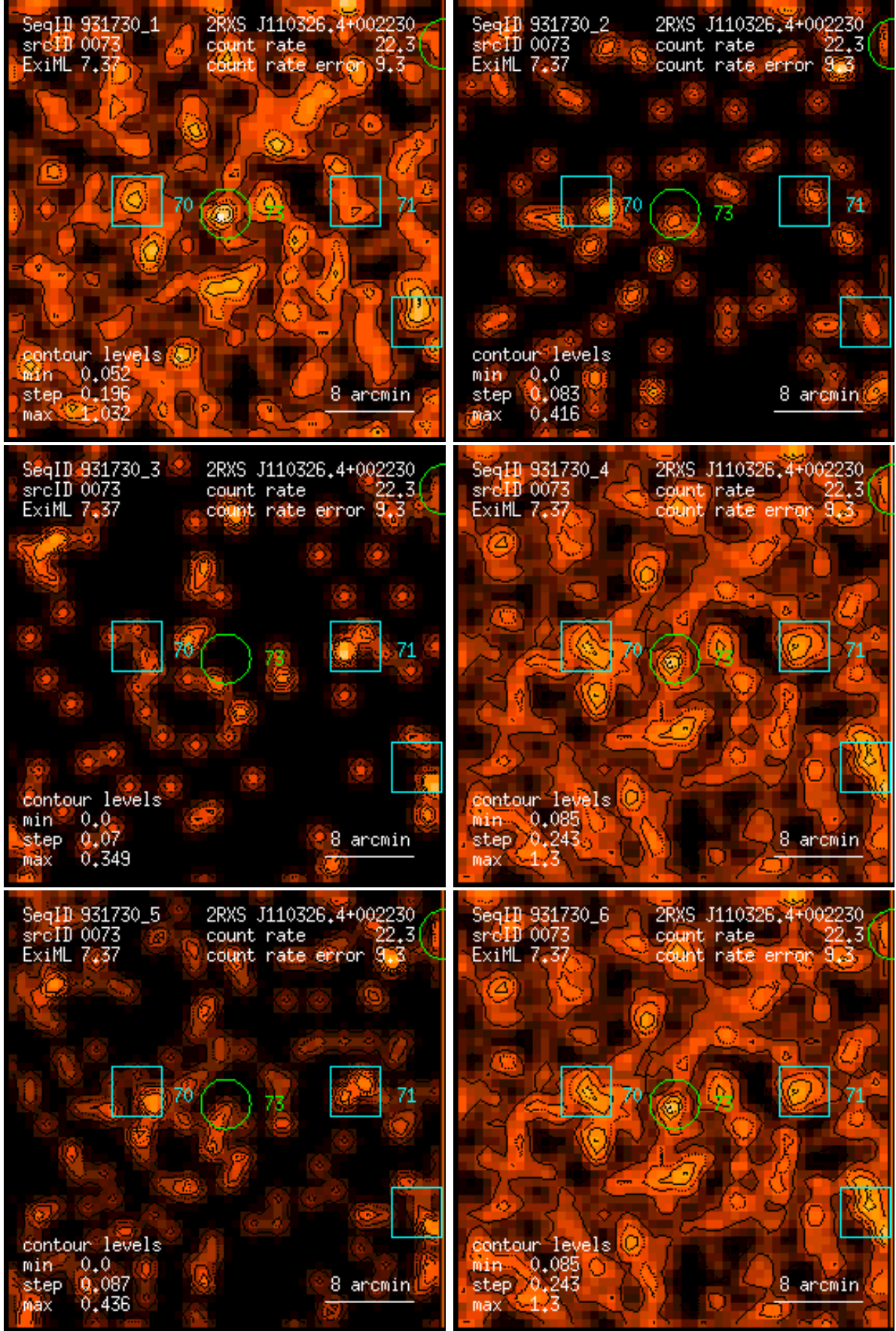
Figure 73: RASS 931730: detection 0073: band rate images, Gaussian filter: (1) PSPC channels 11 – 41, (2) 52 – 90, (3) 91 – 201, (4) 11 – 235, (5) 52 – 201, (6) 11 – 201. Broad band rates in counts/ks. Band rate contour levels in counts/ks/arcmin 2 .
