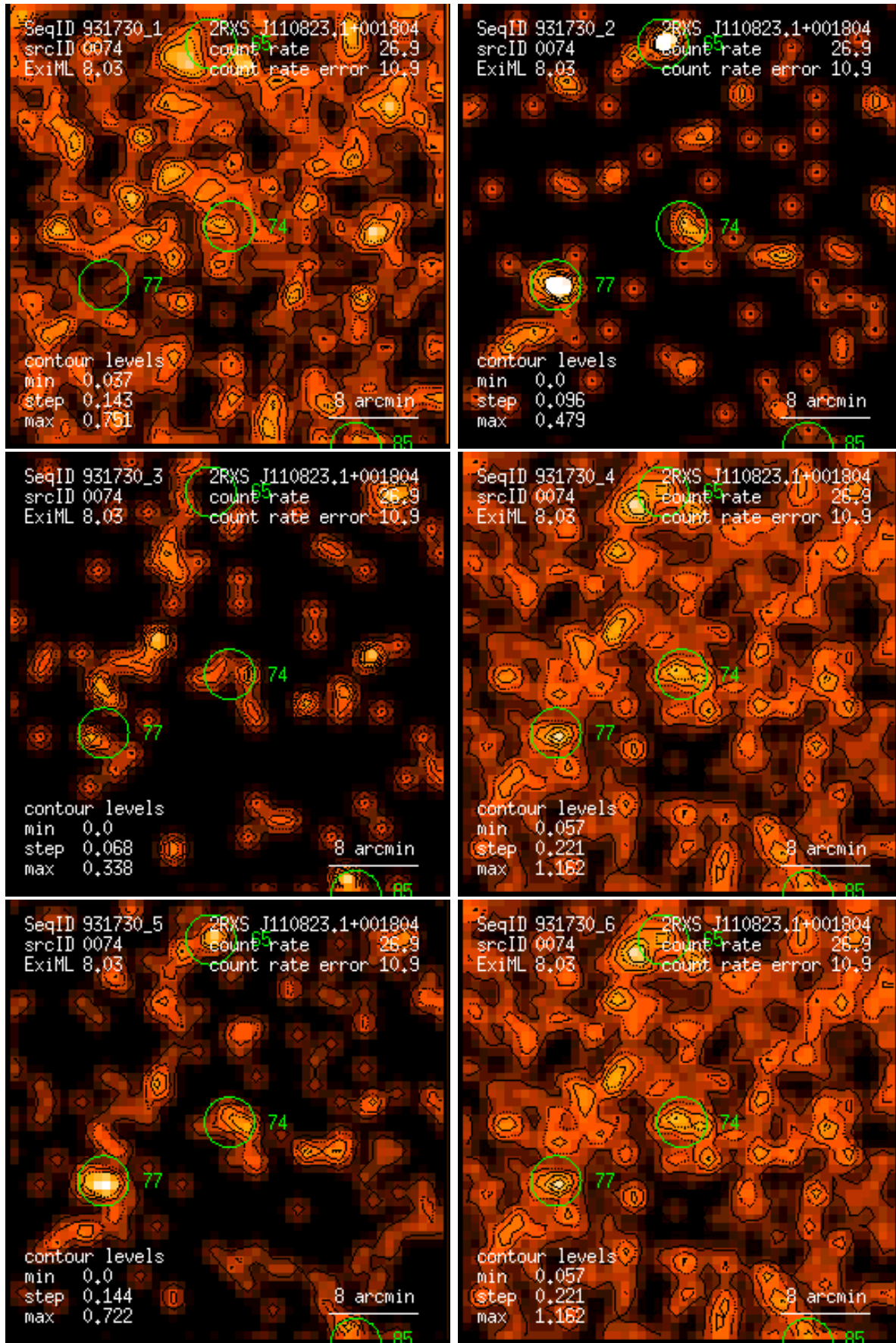
Figure 74: RASS 931730: detection 0074: band rate images, Gaussian filter: (1) PSPC channels 11 – 41, (2) 52 – 90, (3) 91 – 201, (4) 11 – 235, (5) 52 – 201, (6) 11 – 201. Broad band rates in counts/ks. Band rate contour levels in counts/ks/arcmin 2 .
