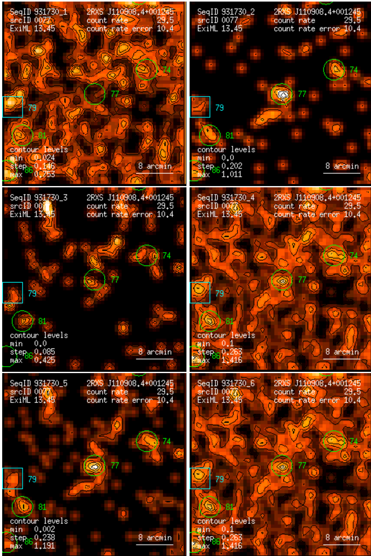
Figure 77: RASS 931730: detection 0077: band rate images, Gaussian filter: (1) PSPC channels 11 – 41, (2) 52 – 90, (3) 91 – 201, (4) 11 – 235, (5) 52 – 201, (6) 11 – 201. Broad band rates in counts/ks. Band rate contour levels in counts/ks/arcmin 2 .
