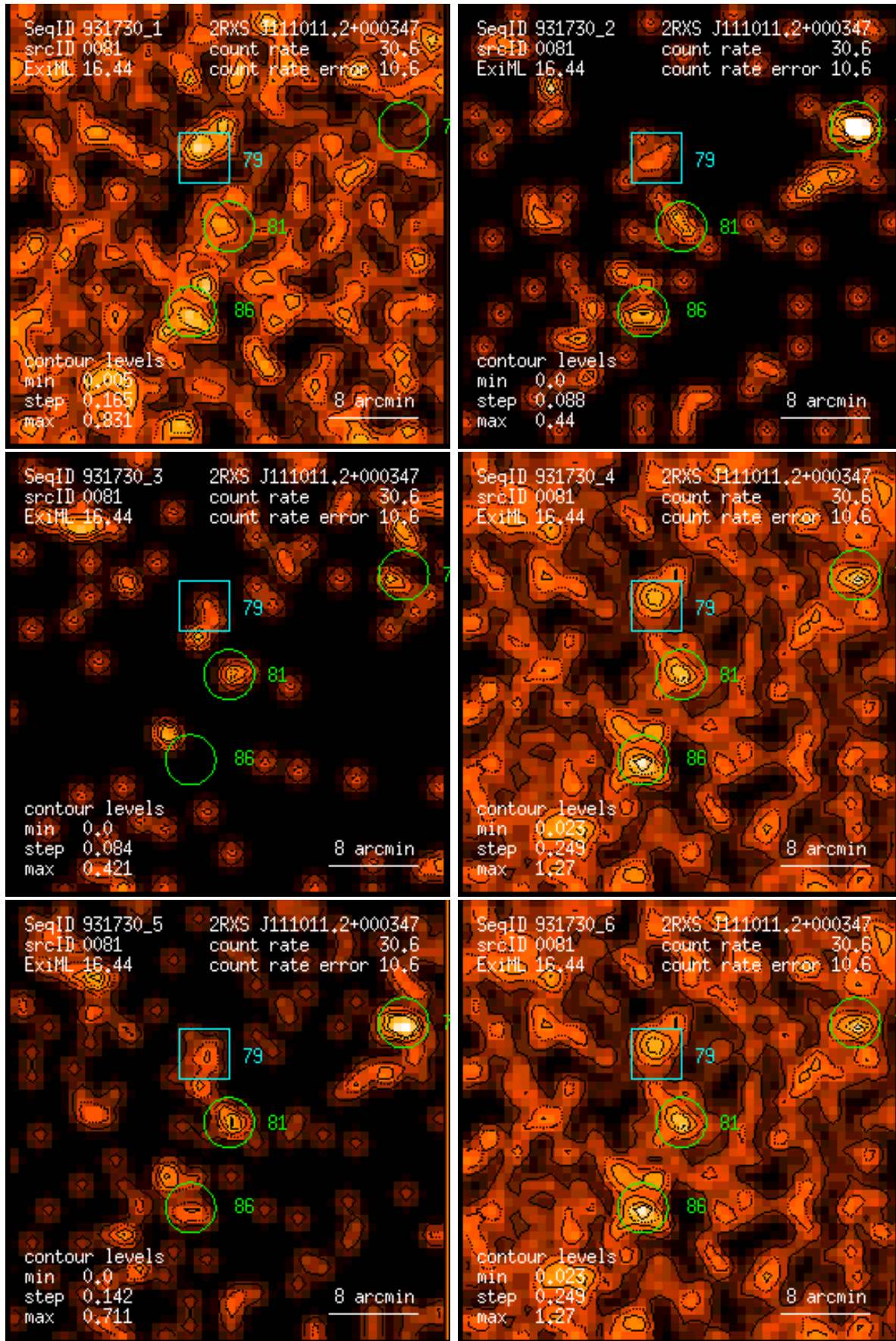
Figure 81: RASS 931730: detection 0081: band rate images, Gaussian filter: (1) PSPC channels 11 – 41, (2) 52 – 90, (3) 91 – 201, (4) 11 – 235, (5) 52 – 201, (6) 11 – 201. Broad band rates in counts/ks. Band rate contour levels in counts/ks/arcmin 2 .
