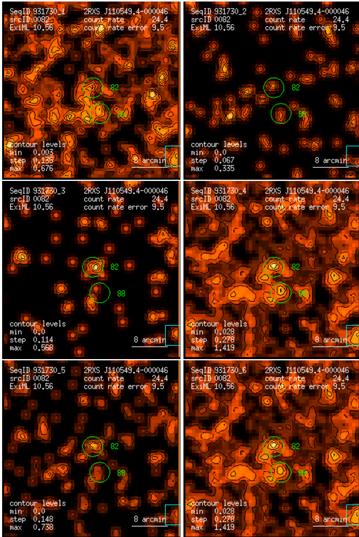
Figure 82: RASS 931730: detection 0082: band rate images, Gaussian filter: (1) PSPC channels 11 – 41, (2) 52 – 90, (3) 91 – 201, (4) 11 – 235, (5) 52 – 201, (6) 11 – 201. Broad band rates in counts/ks. Band rate contour levels in counts/ks/arcmin 2 .
