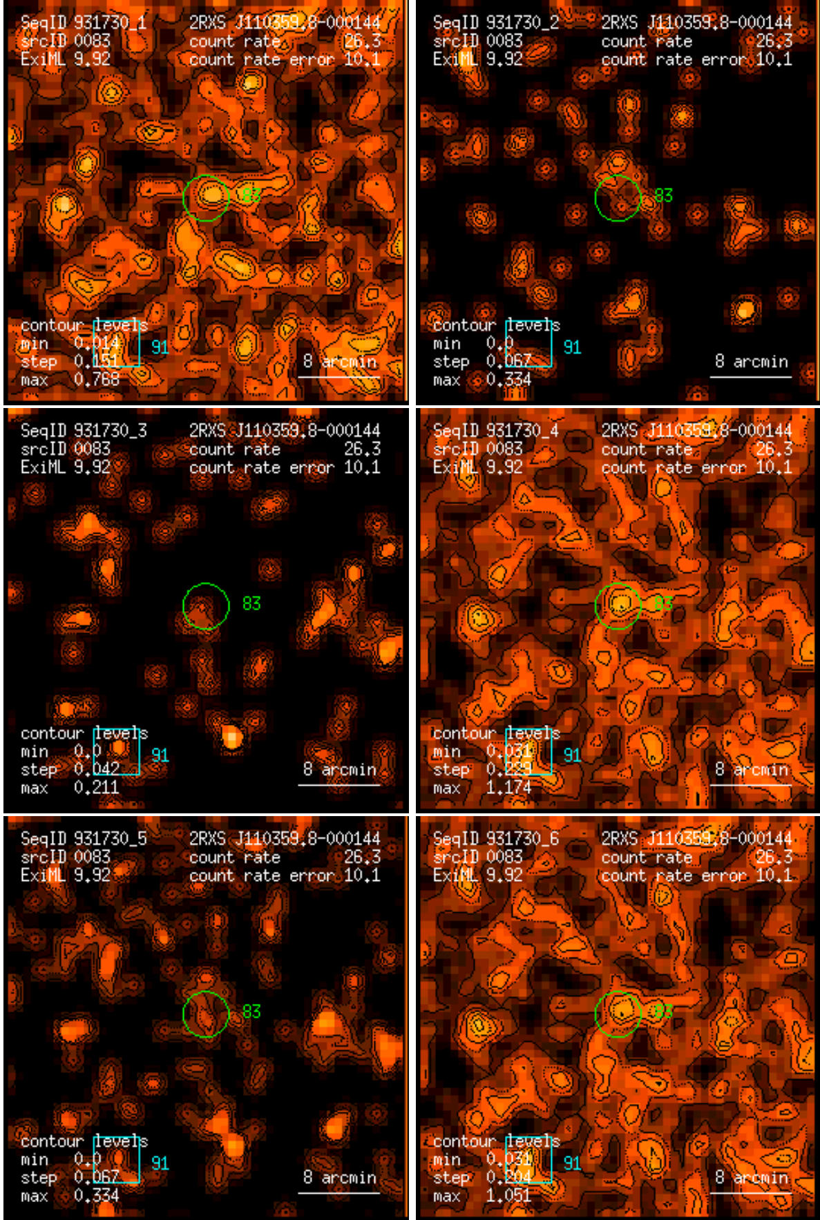
Figure 83: RASS 931730: detection 0083: band rate images, Gaussian filter: (1) PSPC channels 11 – 41, (2) 52 – 90, (3) 91 – 201, (4) 11 – 235, (5) 52 – 201, (6) 11 – 201. Broad band rates in counts/ks. Band rate contour levels in counts/ks/arcmin 2 .
