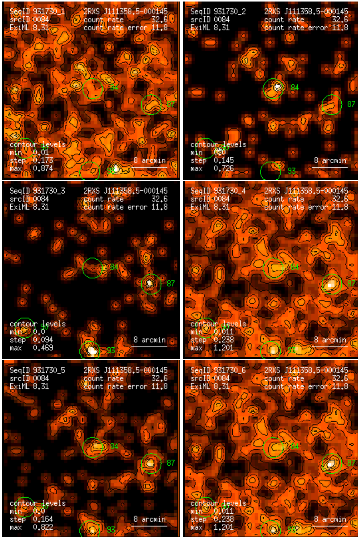
Figure 84: RASS 931730: detection 0084: band rate images, Gaussian filter: (1) PSPC channels 11 – 41, (2) 52 – 90, (3) 91 – 201, (4) 11 – 235, (5) 52 – 201, (6) 11 – 201. Broad band rates in counts/ks. Band rate contour levels in counts/ks/arcmin 2 .
