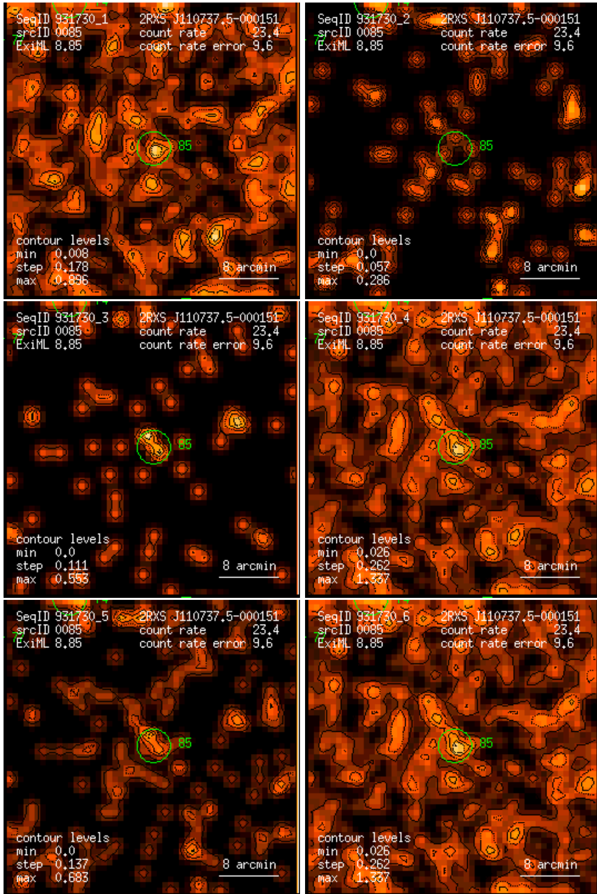
Figure 85: RASS 931730: detection 0085: band rate images, Gaussian filter: (1) PSPC channels 11 – 41, (2) 52 – 90, (3) 91 – 201, (4) 11 – 235, (5) 52 – 201, (6) 11 – 201. Broad band rates in counts/ks. Band rate contour levels in counts/ks/arcmin 2 .
