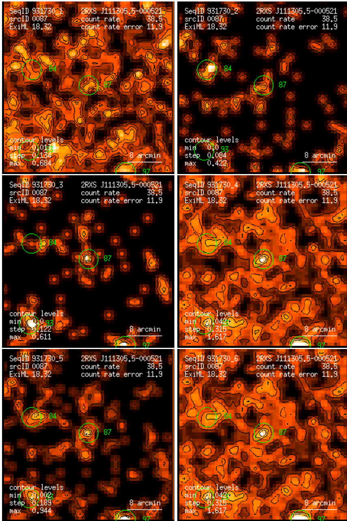
Figure 87: RASS 931730: detection 0087: band rate images, Gaussian filter: (1) PSPC channels 11 – 41, (2) 52 – 90, (3) 91 – 201, (4) 11 – 235, (5) 52 – 201, (6) 11 – 201. Broad band rates in counts/ks. Band rate contour levels in counts/ks/arcmin 2 .
