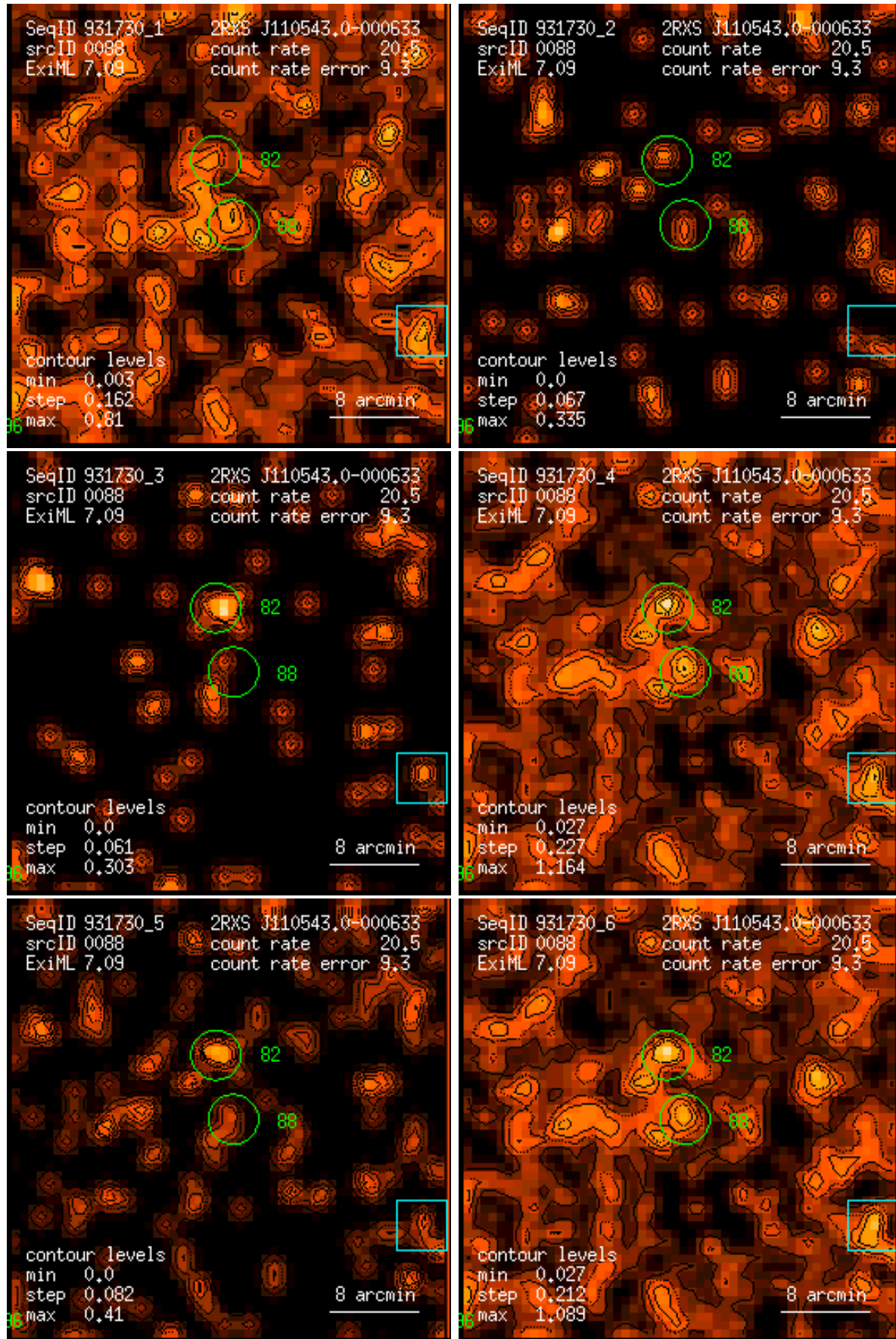
Figure 88: RASS 931730: detection 0088: band rate images, Gaussian filter: (1) PSPC channels 11 – 41, (2) 52 – 90, (3) 91 – 201, (4) 11 – 235, (5) 52 – 201, (6) 11 – 201. Broad band rates in counts/ks. Band rate contour levels in counts/ks/arcmin 2 .
