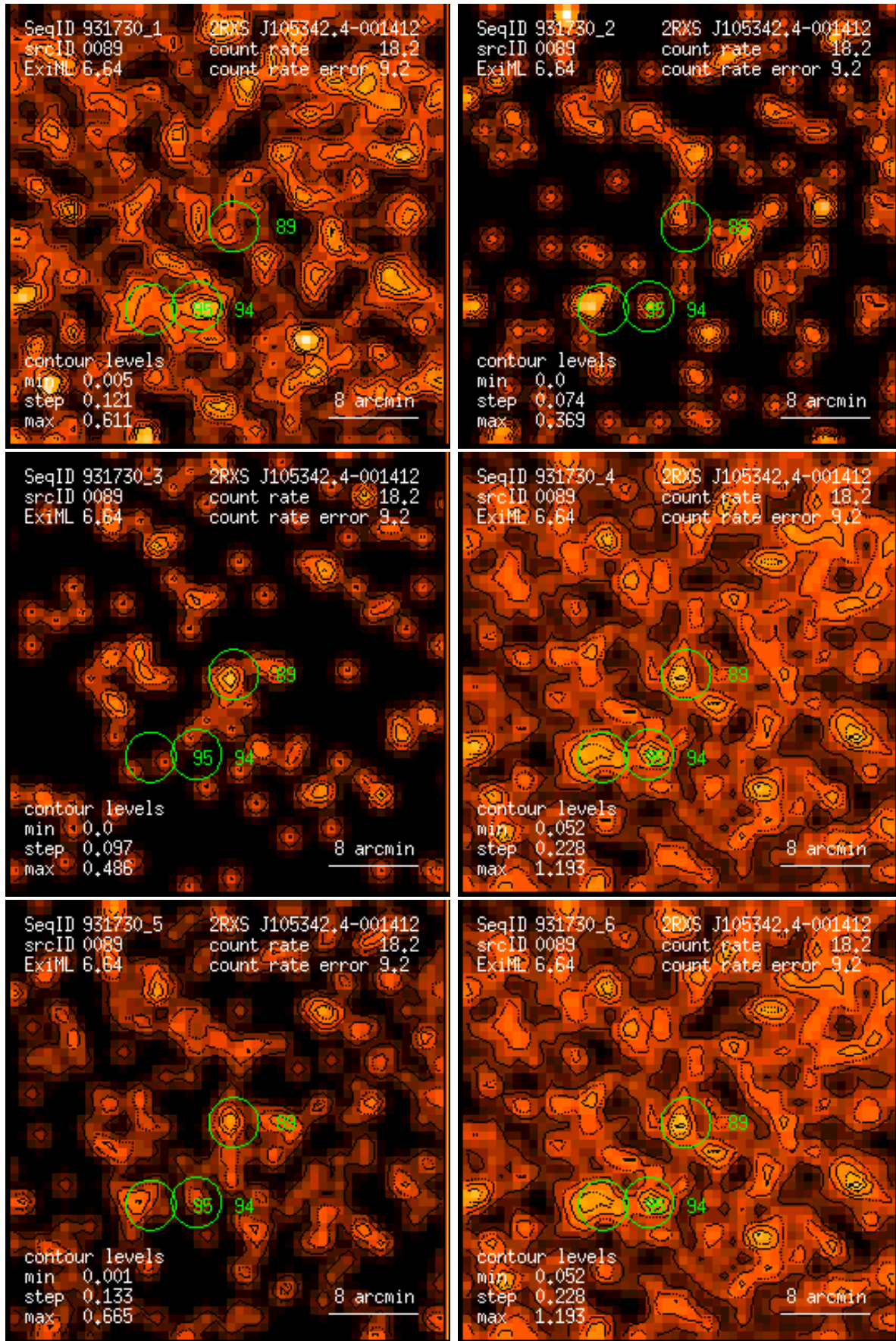
Figure 89: RASS 931730: detection 0089: band rate images, Gaussian filter: (1) PSPC channels 11 – 41, (2) 52 – 90, (3) 91 – 201, (4) 11 – 235, (5) 52 – 201, (6) 11 – 201. Broad band rates in counts/ks. Band rate contour levels in counts/ks/arcmin 2 .
