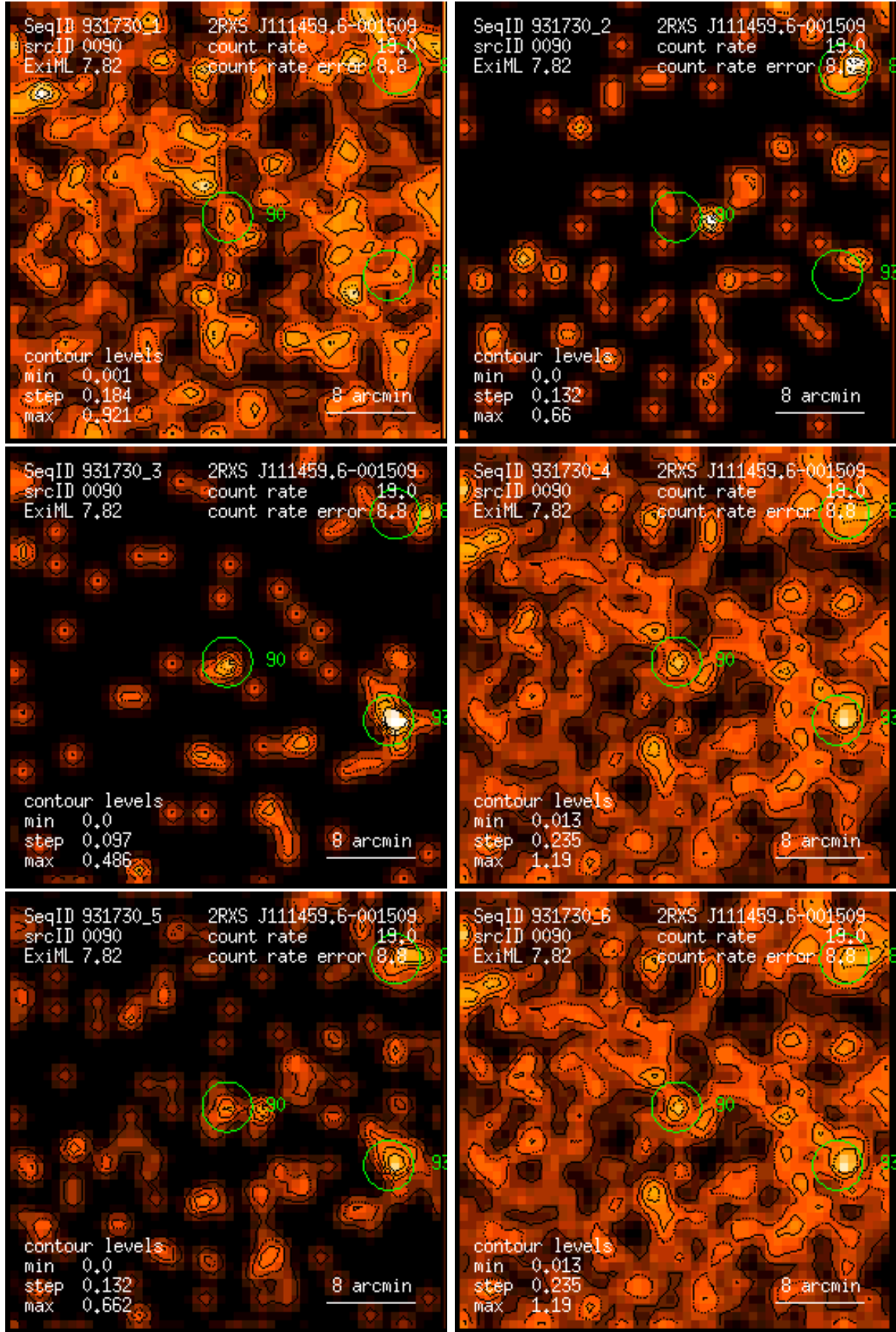
Figure 90: RASS 931730: detection 0090: band rate images, Gaussian filter: (1) PSPC channels 11 – 41, (2) 52 – 90, (3) 91 – 201, (4) 11 – 235, (5) 52 – 201, (6) 11 – 201. Broad band rates in counts/ks. Band rate contour levels in counts/ks/arcmin 2 .
