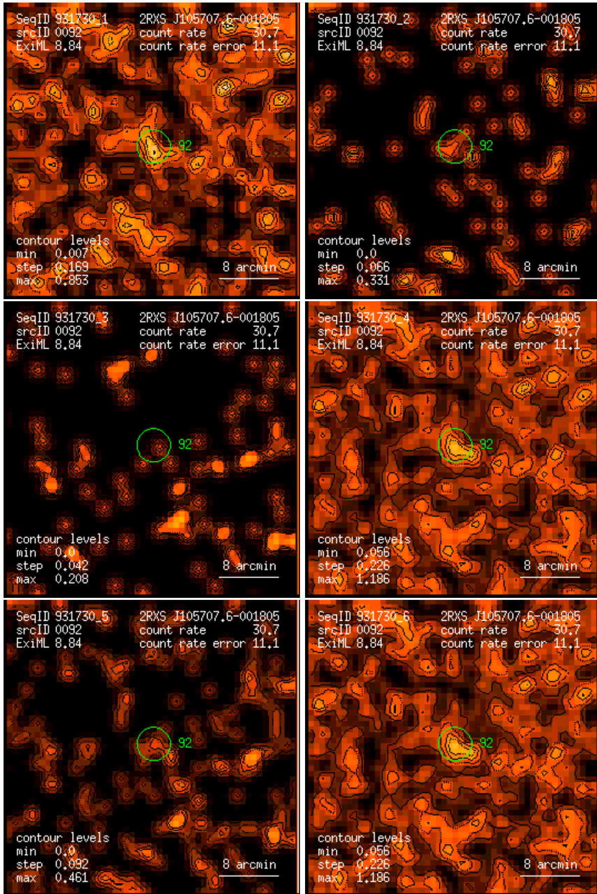
Figure 92: RASS 931730: detection 0092: band rate images, Gaussian filter: (1) PSPC channels 11 – 41, (2) 52 – 90, (3) 91 – 201, (4) 11 – 235, (5) 52 – 201, (6) 11 – 201. Broad band rates in counts/ks. Band rate contour levels in counts/ks/arcmin 2 .
