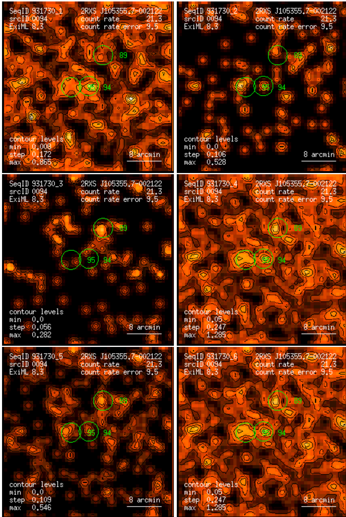
Figure 94: RASS 931730: detection 0094: band rate images, Gaussian filter: (1) PSPC channels 11 – 41, (2) 52 – 90, (3) 91 – 201, (4) 11 – 235, (5) 52 – 201, (6) 11 – 201. Broad band rates in counts/ks. Band rate contour levels in counts/ks/arcmin 2 .
