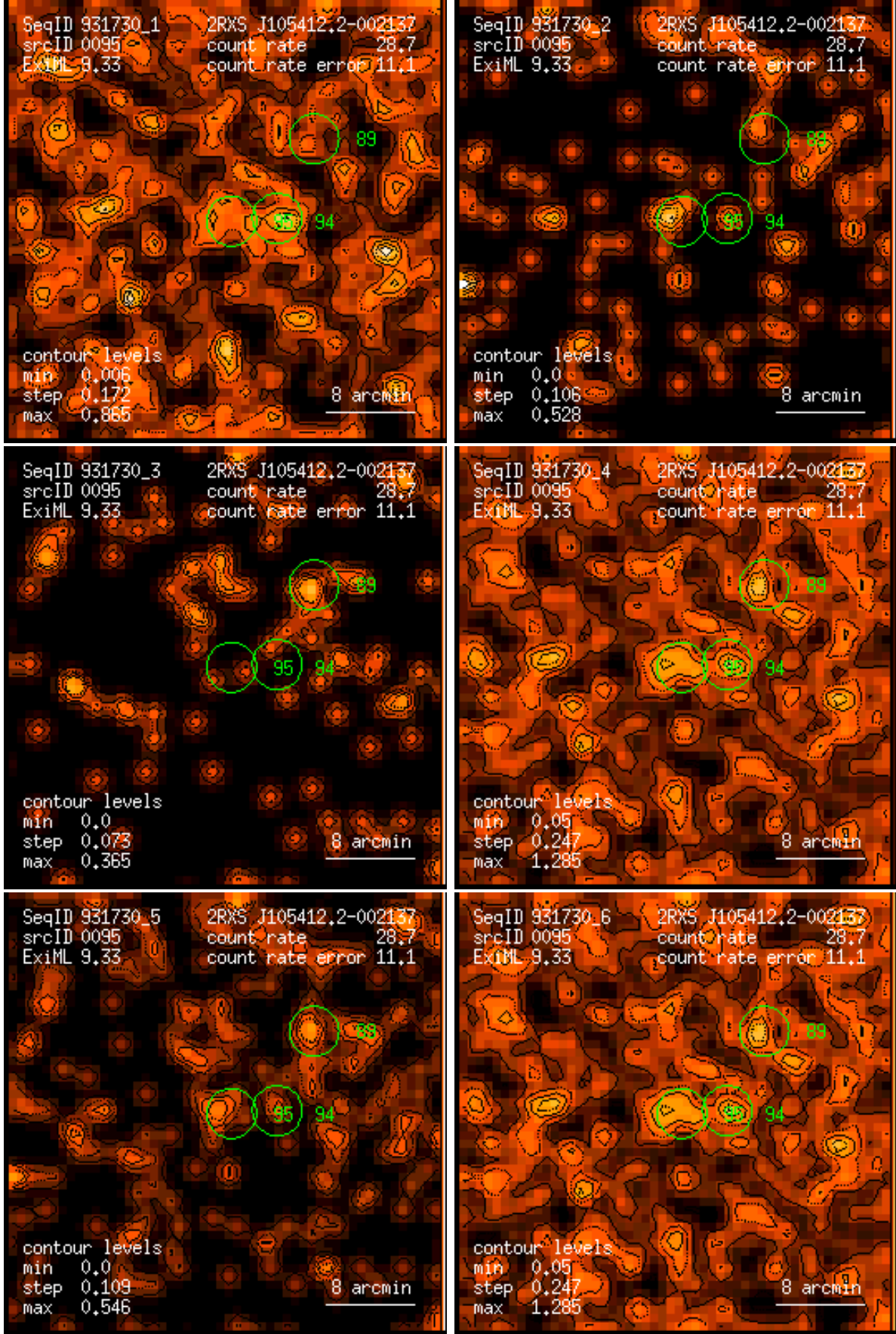
Figure 95: RASS 931730: detection 0095: band rate images, Gaussian filter: (1) PSPC channels 11 – 41, (2) 52 – 90, (3) 91 – 201, (4) 11 – 235, (5) 52 – 201, (6) 11 – 201. Broad band rates in counts/ks. Band rate contour levels in counts/ks/arcmin 2 .
