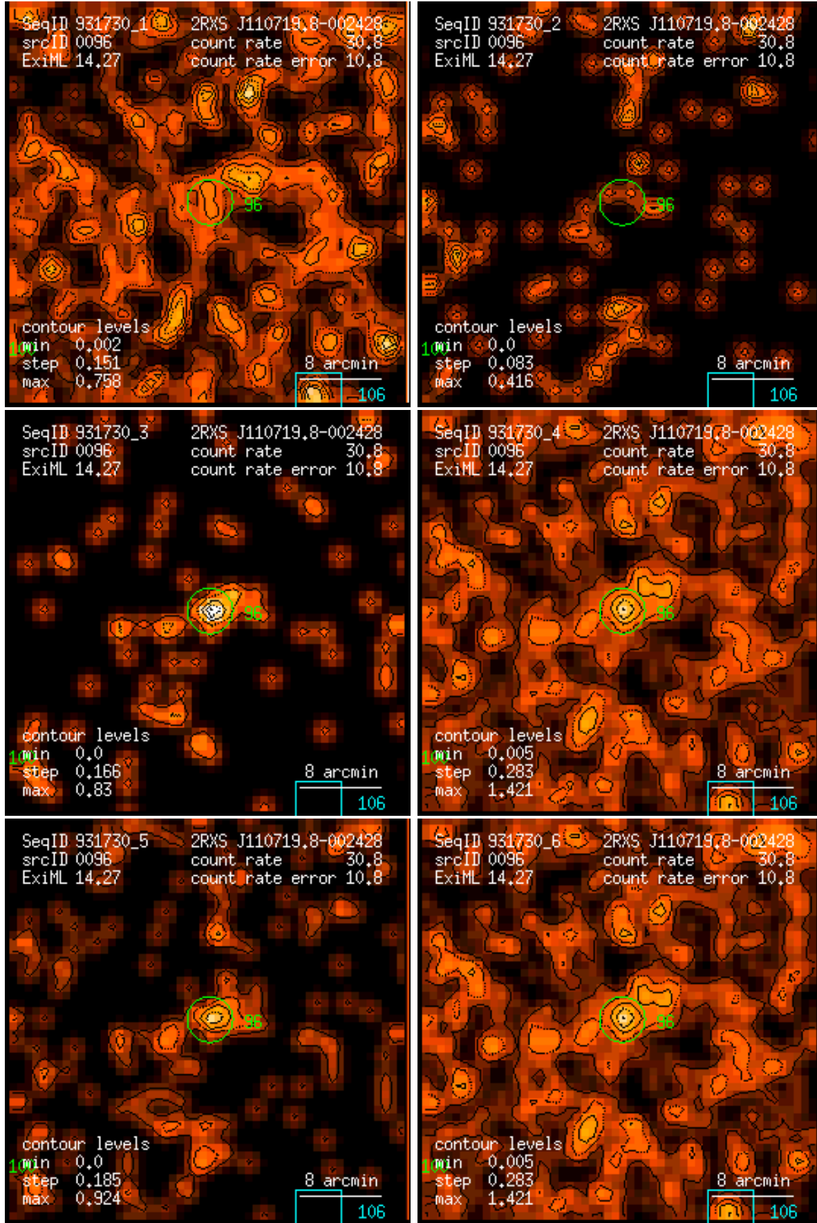
Figure 96: RASS 931730: detection 0096: band rate images, Gaussian filter: (1) PSPC channels 11 – 41, (2) 52 – 90, (3) 91 – 201, (4) 11 – 235, (5) 52 – 201, (6) 11 – 201. Broad band rates in counts/ks. Band rate contour levels in counts/ks/arcmin 2 .
