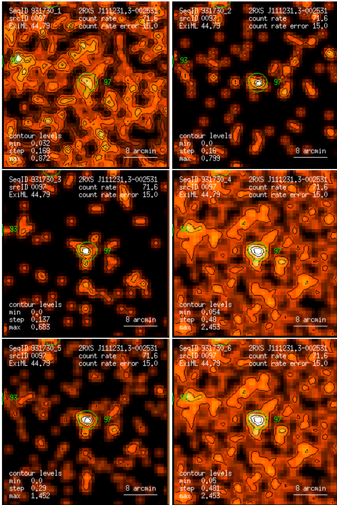
Figure 97: RASS 931730: detection 0097: band rate images, Gaussian filter: (1) PSPC channels 11 – 41, (2) 52 – 90, (3) 91 – 201, (4) 11 – 235, (5) 52 – 201, (6) 11 – 201. Broad band rates in counts/ks. Band rate contour levels in counts/ks/arcmin 2 .
