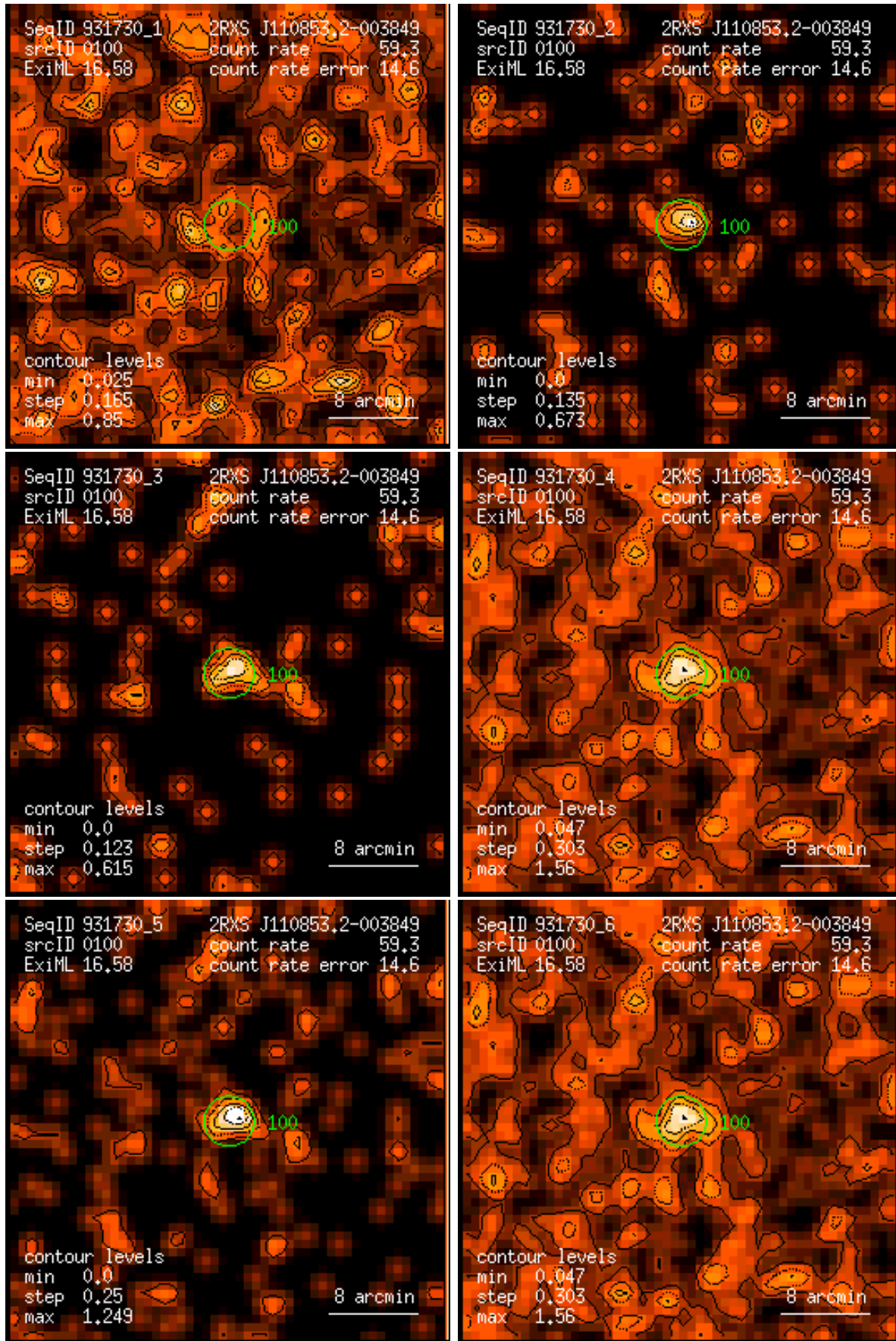
Figure 100: RASS 931730: detection 0100: band rate images, Gaussian filter: (1) PSPC channels 11 – 41, (2) 52 – 90, (3) 91 – 201, (4) 11 – 235, (5) 52 – 201, (6) 11 – 201. Broad band rates in counts/ks. Band rate contour levels in counts/ks/arcmin 2 .
