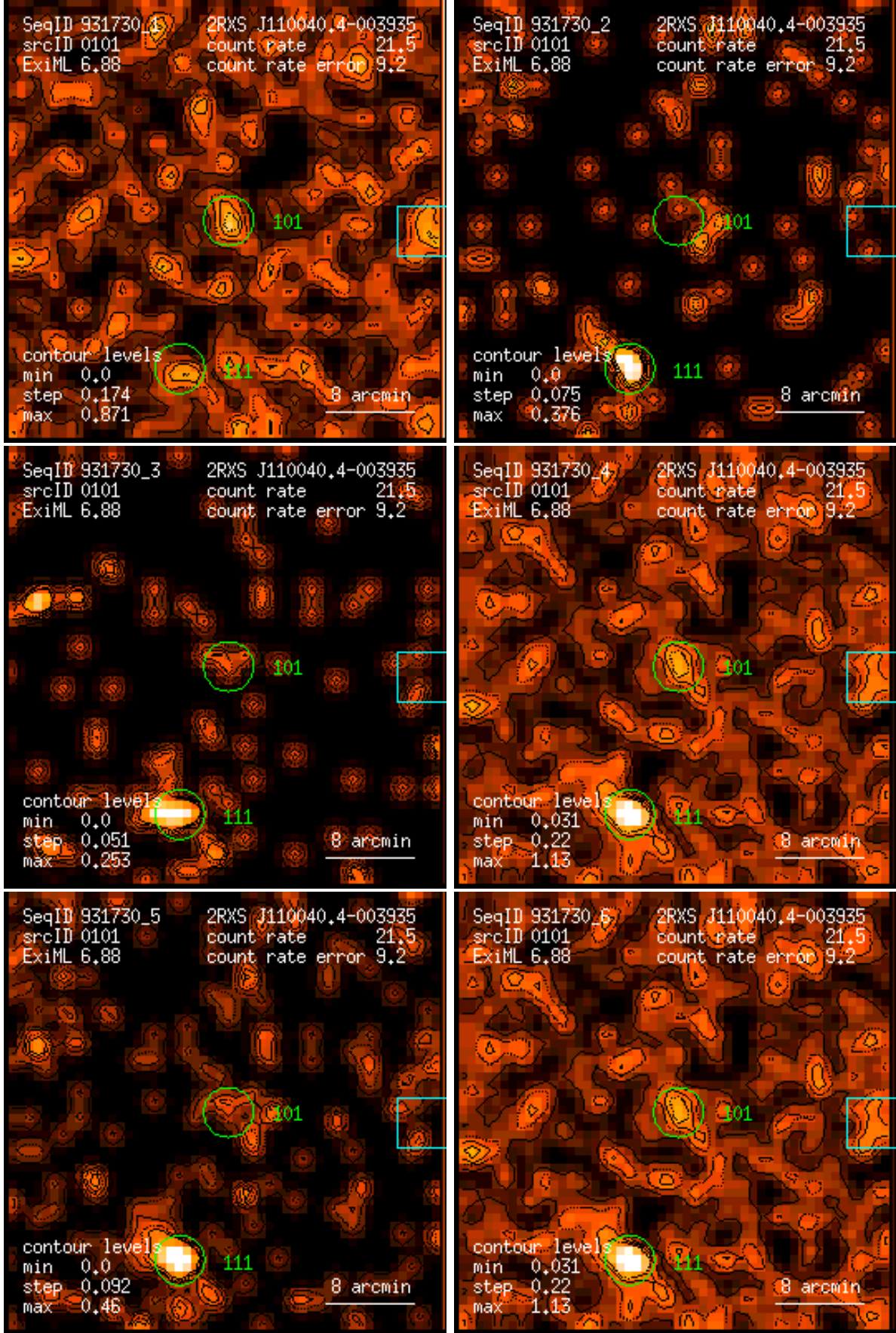
Figure 101: RASS 931730: detection 0101: band rate images, Gaussian filter: (1) PSPC channels 11 – 41, (2) 52 – 90, (3) 91 – 201, (4) 11 – 235, (5) 52 – 201, (6) 11 – 201. Broad band rates in counts/ks. Band rate contour levels in counts/ks/arcmin 2 .
