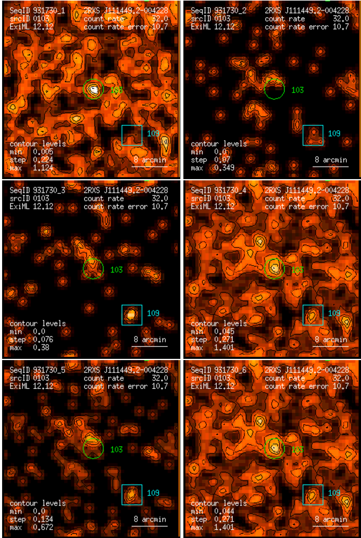
Figure 103: RASS 931730: detection 0103: band rate images, Gaussian filter: (1) PSPC channels 11 – 41, (2) 52 – 90, (3) 91 – 201, (4) 11 – 235, (5) 52 – 201, (6) 11 – 201. Broad band rates in counts/ks. Band rate contour levels in counts/ks/arcmin 2 .
