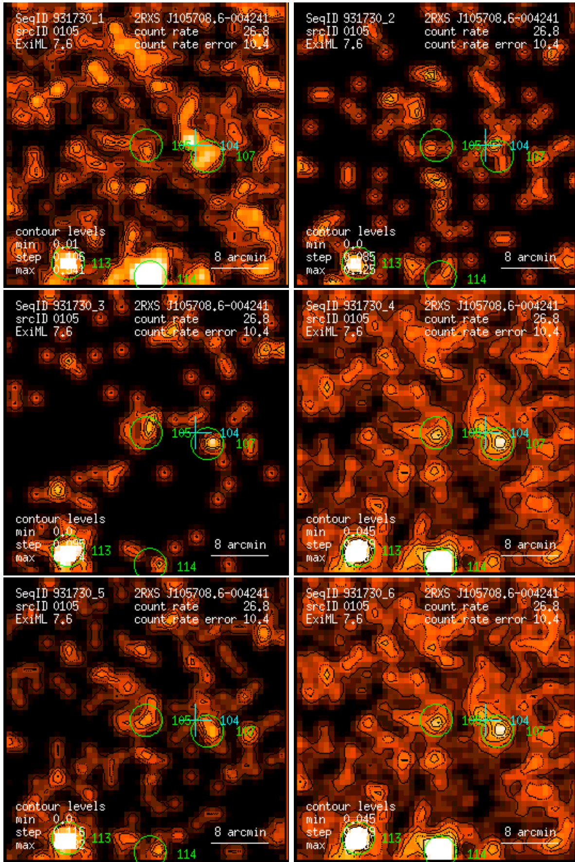
Figure 105: RASS 931730: detection 0105: band rate images, Gaussian filter: (1) PSPC channels 11 – 41, (2) 52 – 90, (3) 91 – 201, (4) 11 – 235, (5) 52 – 201, (6) 11 – 201. Broad band rates in counts/ks. Band rate contour levels in counts/ks/arcmin 2 .
