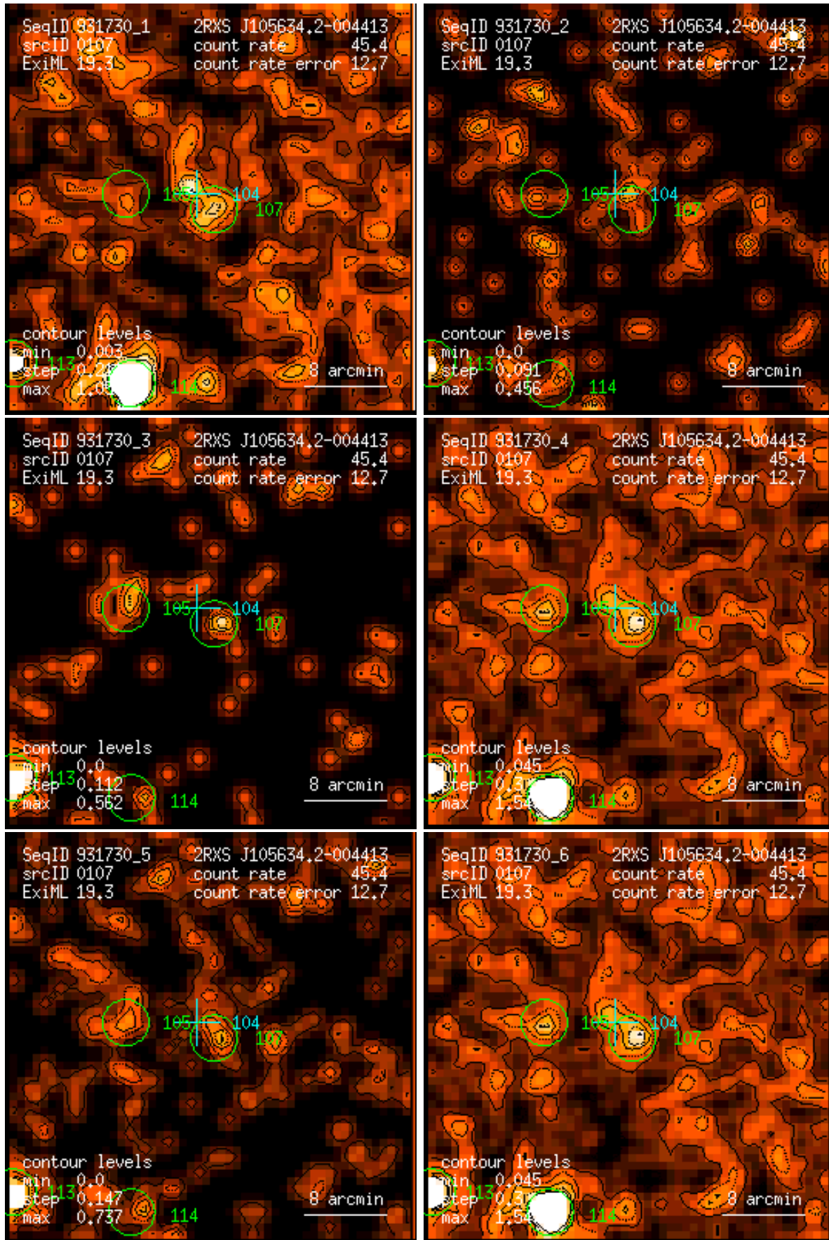
Figure 107: RASS 931730: detection 0107: band rate images, Gaussian filter: (1) PSPC channels 11 – 41, (2) 52 – 90, (3) 91 – 201, (4) 11 – 235, (5) 52 – 201, (6) 11 – 201. Broad band rates in counts/ks. Band rate contour levels in counts/ks/arcmin 2 .
