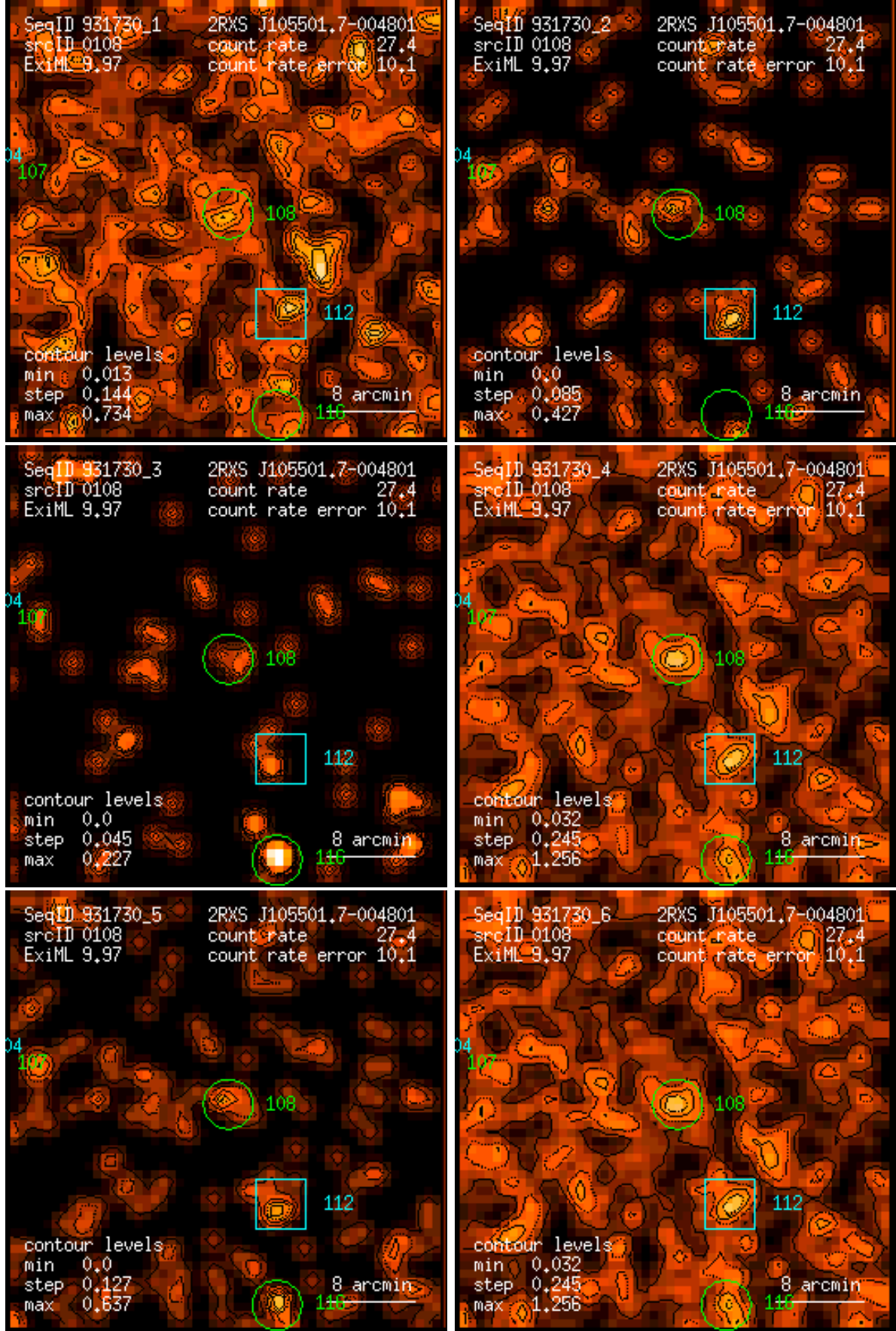
Figure 108: RASS 931730: detection 0108: band rate images, Gaussian filter: (1) PSPC channels 11 – 41, (2) 52 – 90, (3) 91 – 201, (4) 11 – 235, (5) 52 – 201, (6) 11 – 201. Broad band rates in counts/ks. Band rate contour levels in counts/ks/arcmin 2 .
