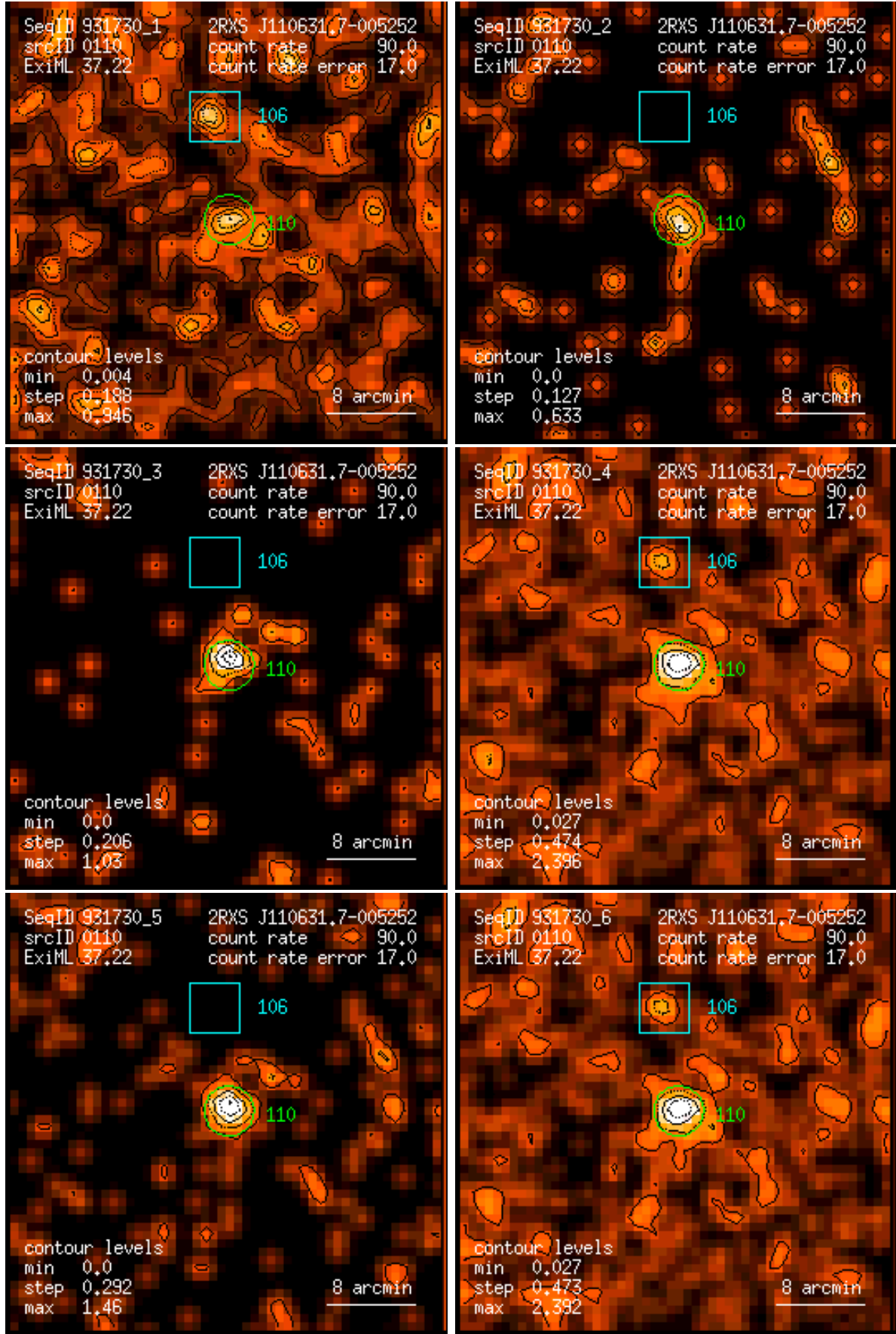
Figure 110: RASS 931730: detection 0110: band rate images, Gaussian filter: (1) PSPC channels 11 – 41, (2) 52 – 90, (3) 91 – 201, (4) 11 – 235, (5) 52 – 201, (6) 11 – 201. Broad band rates in counts/ks. Band rate contour levels in counts/ks/arcmin 2 .
