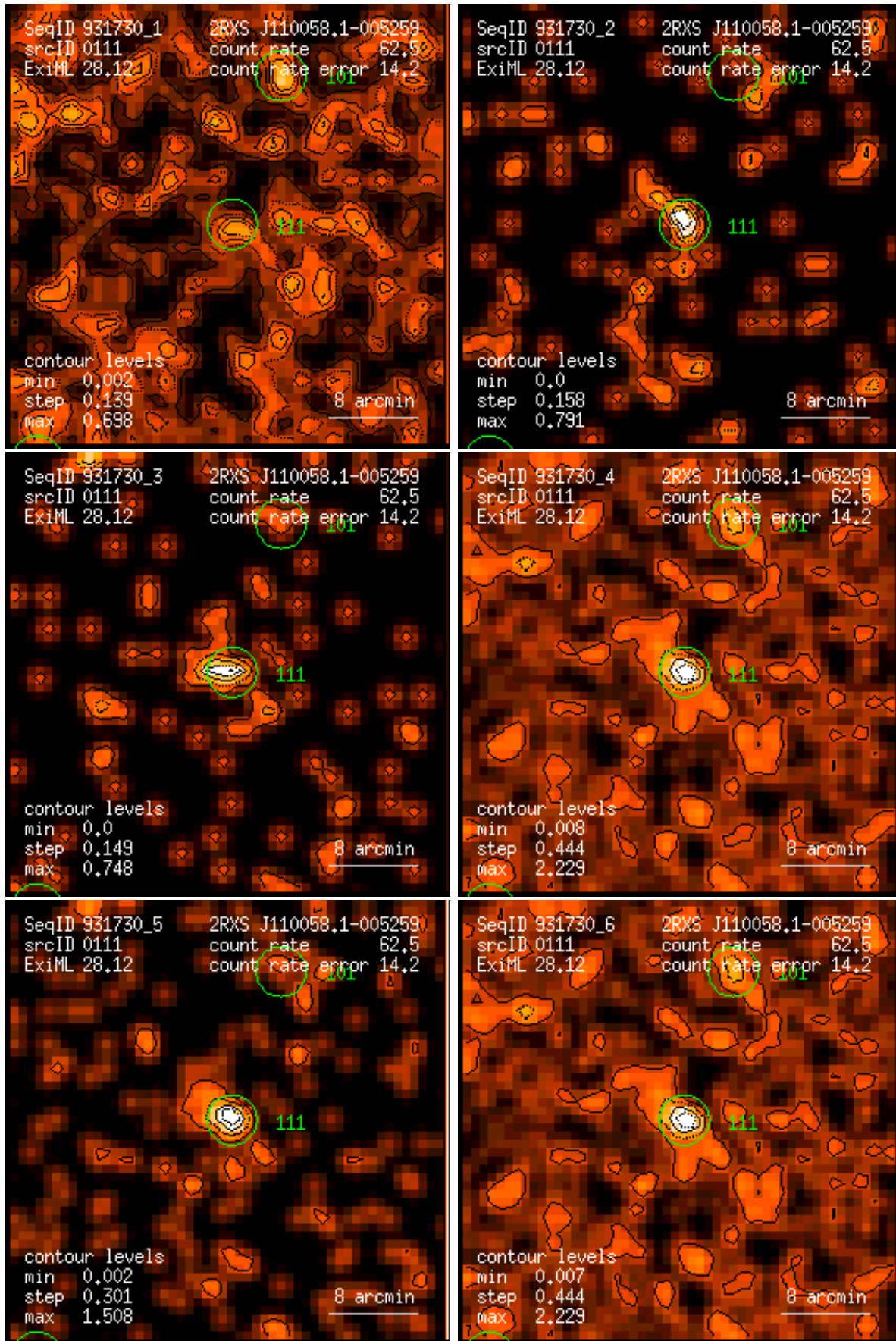
Figure 111: RASS 931730: detection 0111: band rate images, Gaussian filter: (1) PSPC channels 11 – 41, (2) 52 – 90, (3) 91 – 201, (4) 11 – 235, (5) 52 – 201, (6) 11 – 201. Broad band rates in counts/ks. Band rate contour levels in counts/ks/arcmin 2 .
