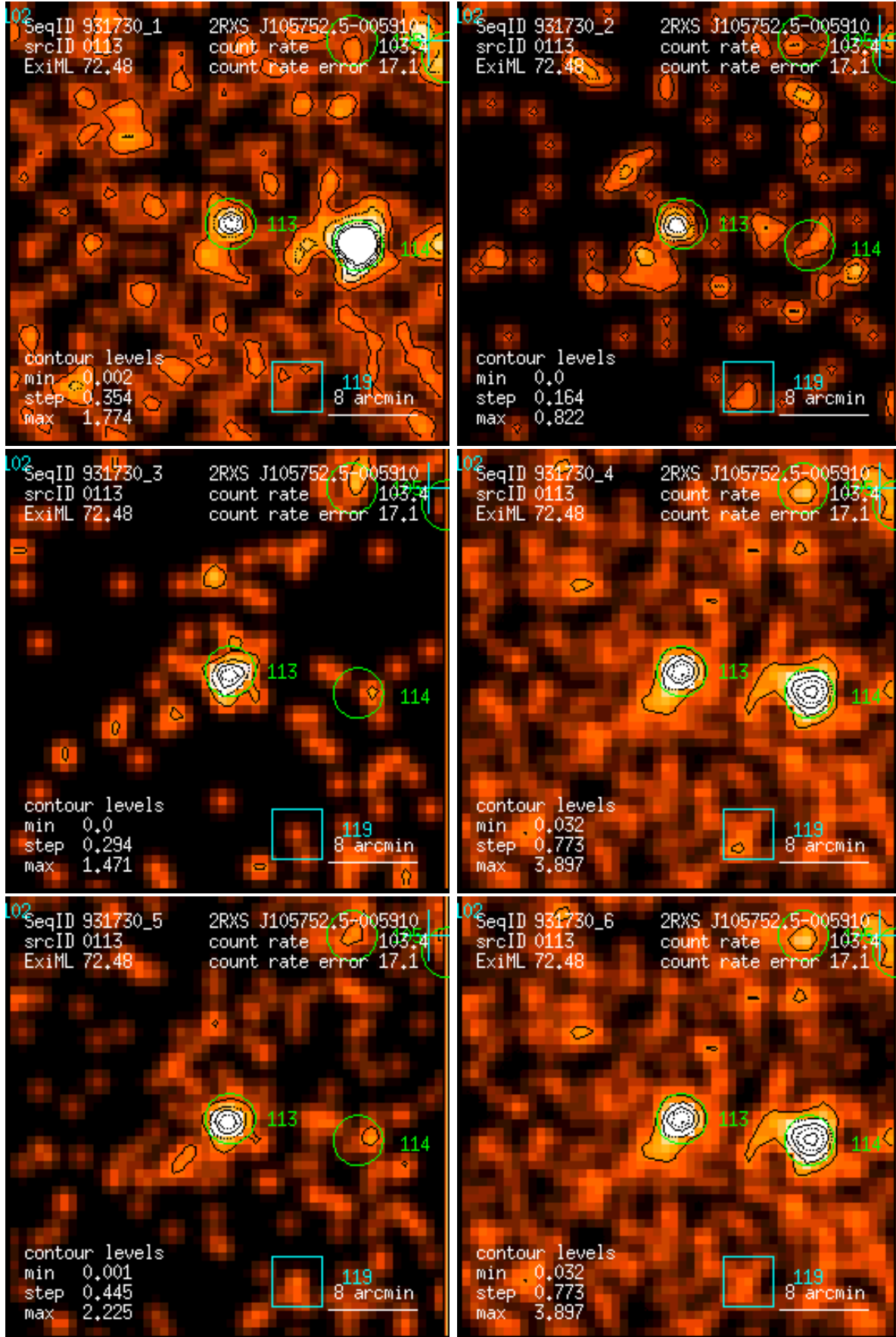
Figure 113: RASS 931730: detection 0113: band rate images, Gaussian filter: (1) PSPC channels 11 – 41, (2) 52 – 90, (3) 91 – 201, (4) 11 – 235, (5) 52 – 201, (6) 11 – 201. Broad band rates in counts/ks. Band rate contour levels in counts/ks/arcmin 2 .
