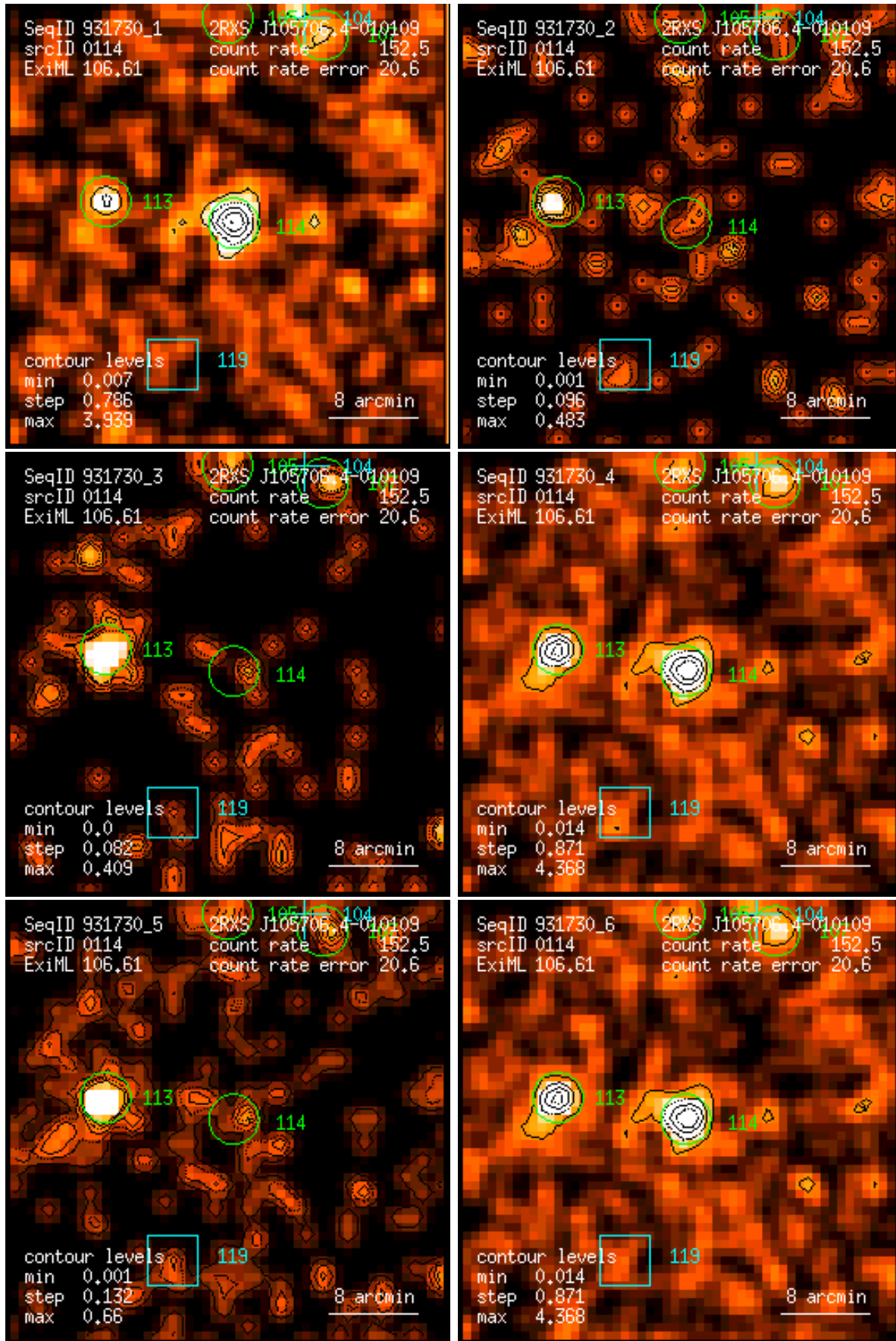
Figure 114: RASS 931730: detection 0114: band rate images, Gaussian filter: (1) PSPC channels 11 – 41, (2) 52 – 90, (3) 91 – 201, (4) 11 – 235, (5) 52 – 201, (6) 11 – 201. Broad band rates in counts/ks. Band rate contour levels in counts/ks/arcmin 2 .
