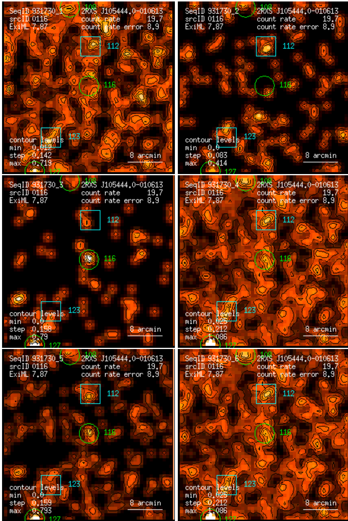
Figure 116: RASS 931730: detection 0116: band rate images, Gaussian filter: (1) PSPC channels 11 – 41, (2) 52 – 90, (3) 91 – 201, (4) 11 – 235, (5) 52 – 201, (6) 11 – 201. Broad band rates in counts/ks. Band rate contour levels in counts/ks/arcmin 2 .
