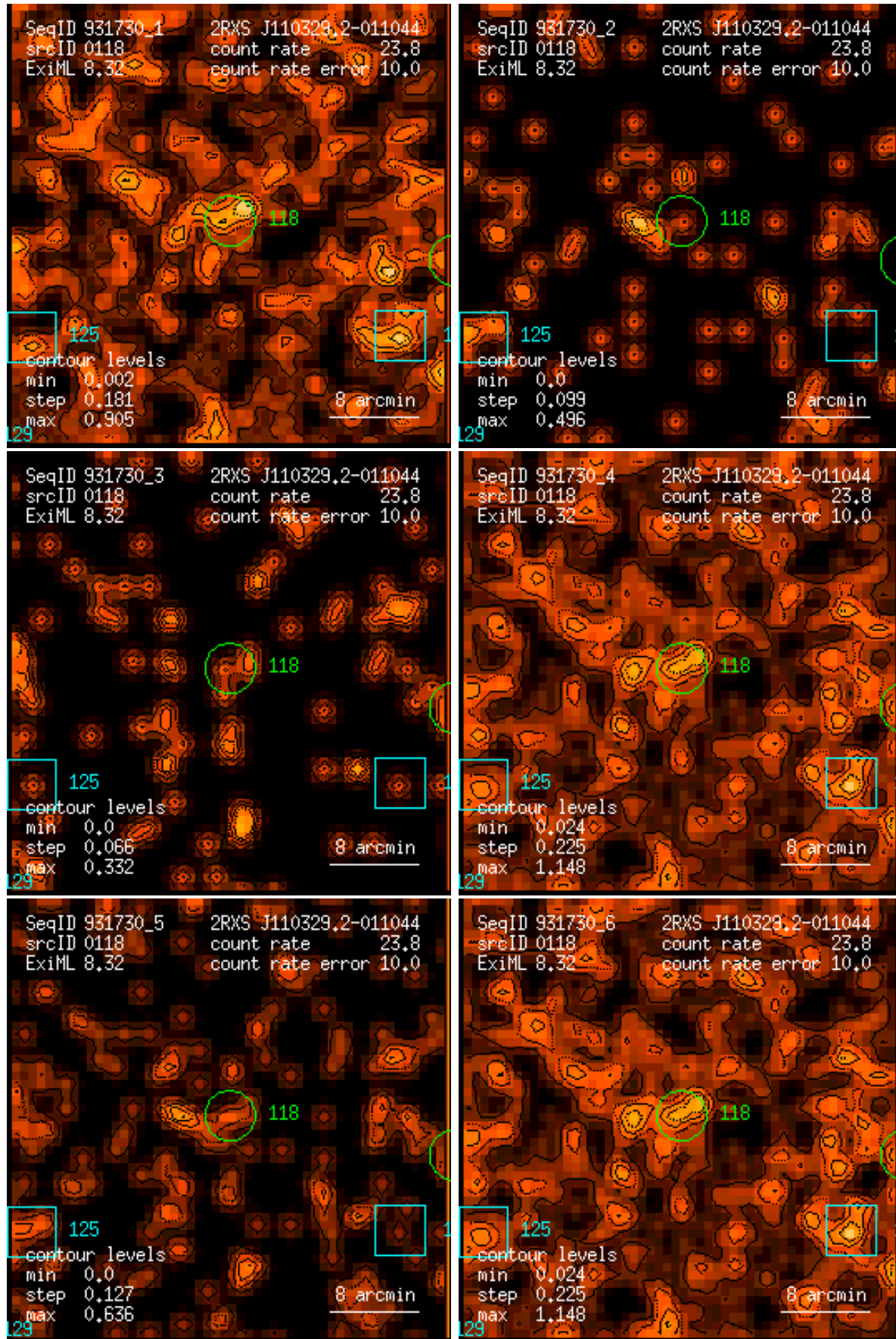
Figure 118: RASS 931730: detection 0118: band rate images, Gaussian filter: (1) PSPC channels 11 – 41, (2) 52 – 90, (3) 91 – 201, (4) 11 – 235, (5) 52 – 201, (6) 11 – 201. Broad band rates in counts/ks. Band rate contour levels in counts/ks/arcmin 2 .
