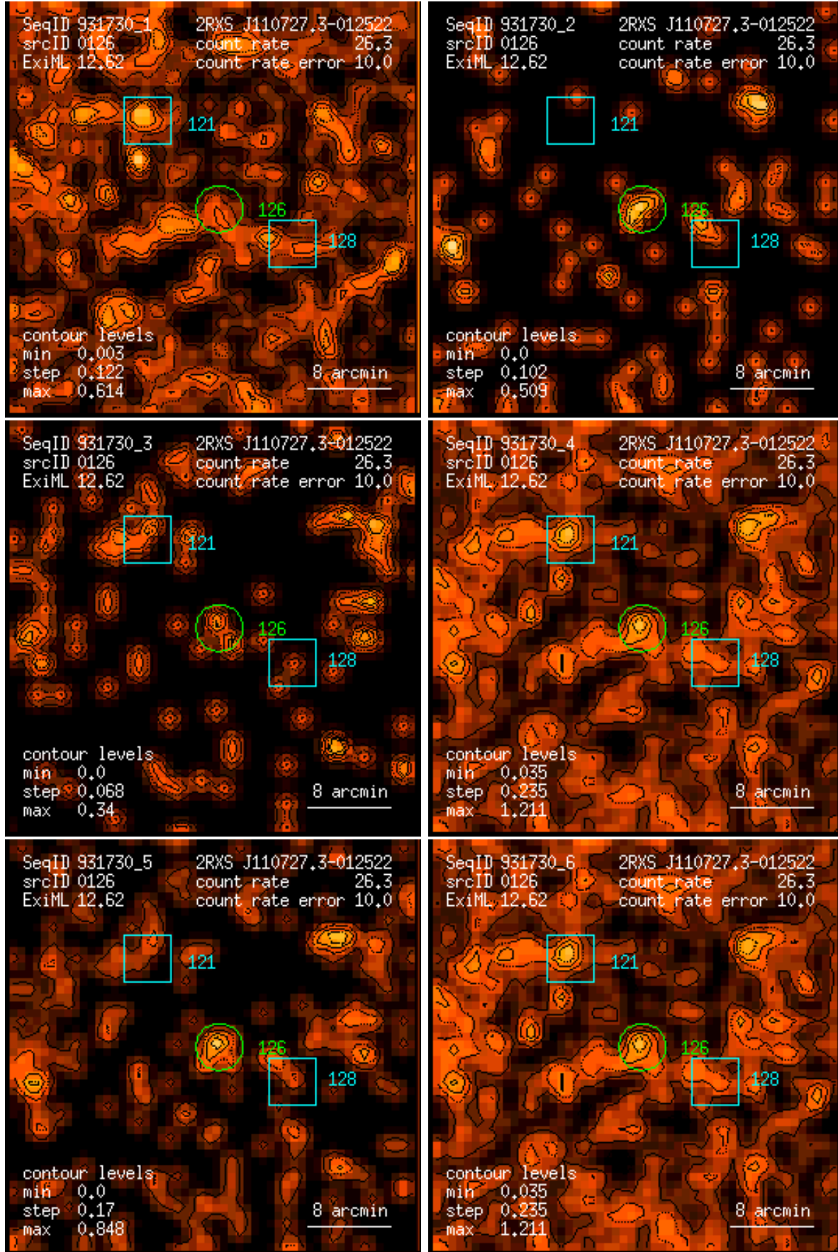
Figure 126: RASS 931730: detection 0126: band rate images, Gaussian filter: (1) PSPC channels 11 – 41, (2) 52 – 90, (3) 91 – 201, (4) 11 – 235, (5) 52 – 201, (6) 11 – 201. Broad band rates in counts/ks. Band rate contour levels in counts/ks/arcmin 2 .
