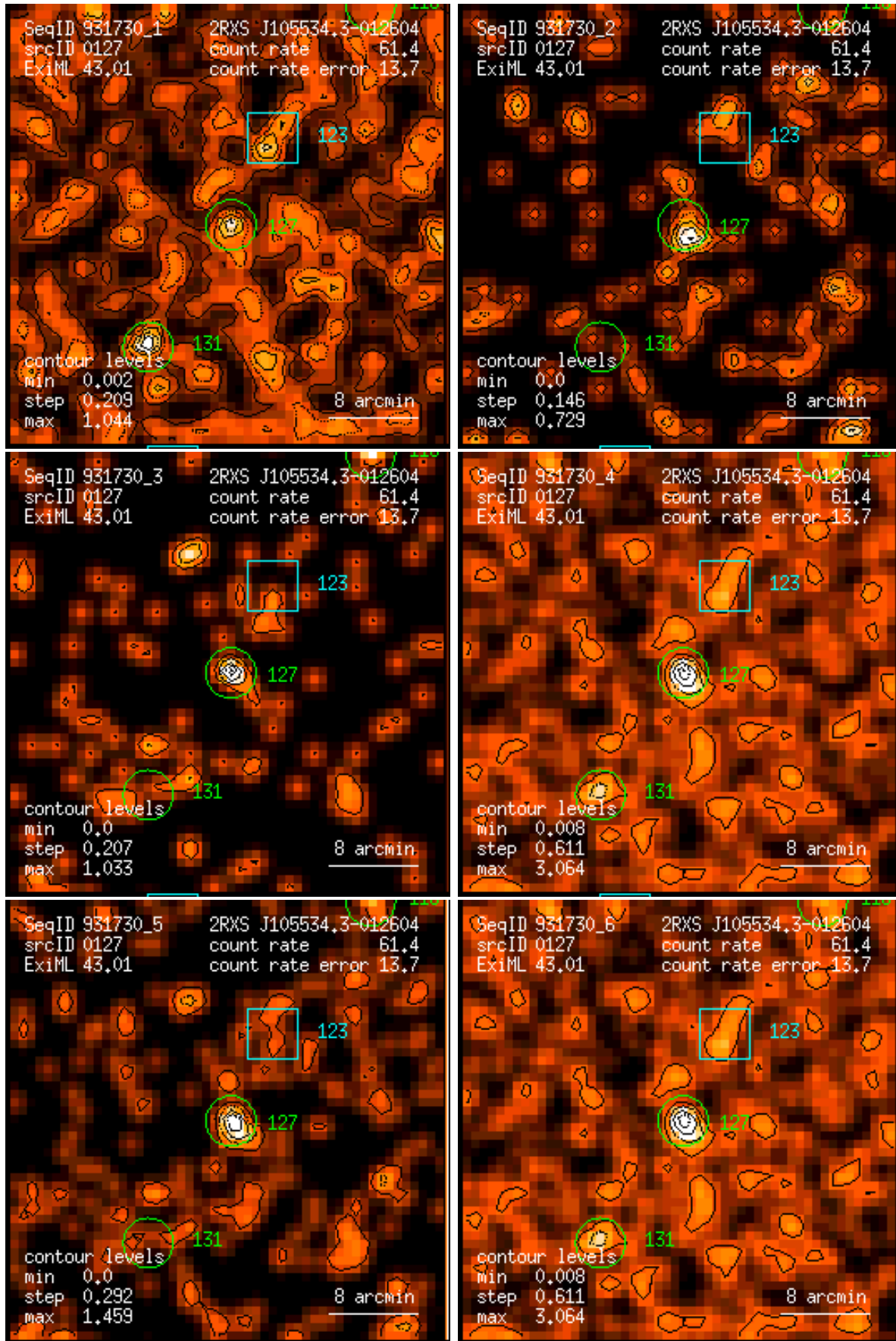
Figure 127: RASS 931730: detection 0127: band rate images, Gaussian filter: (1) PSPC channels 11 – 41, (2) 52 – 90, (3) 91 – 201, (4) 11 – 235, (5) 52 – 201, (6) 11 – 201. Broad band rates in counts/ks. Band rate contour levels in counts/ks/arcmin 2 .
