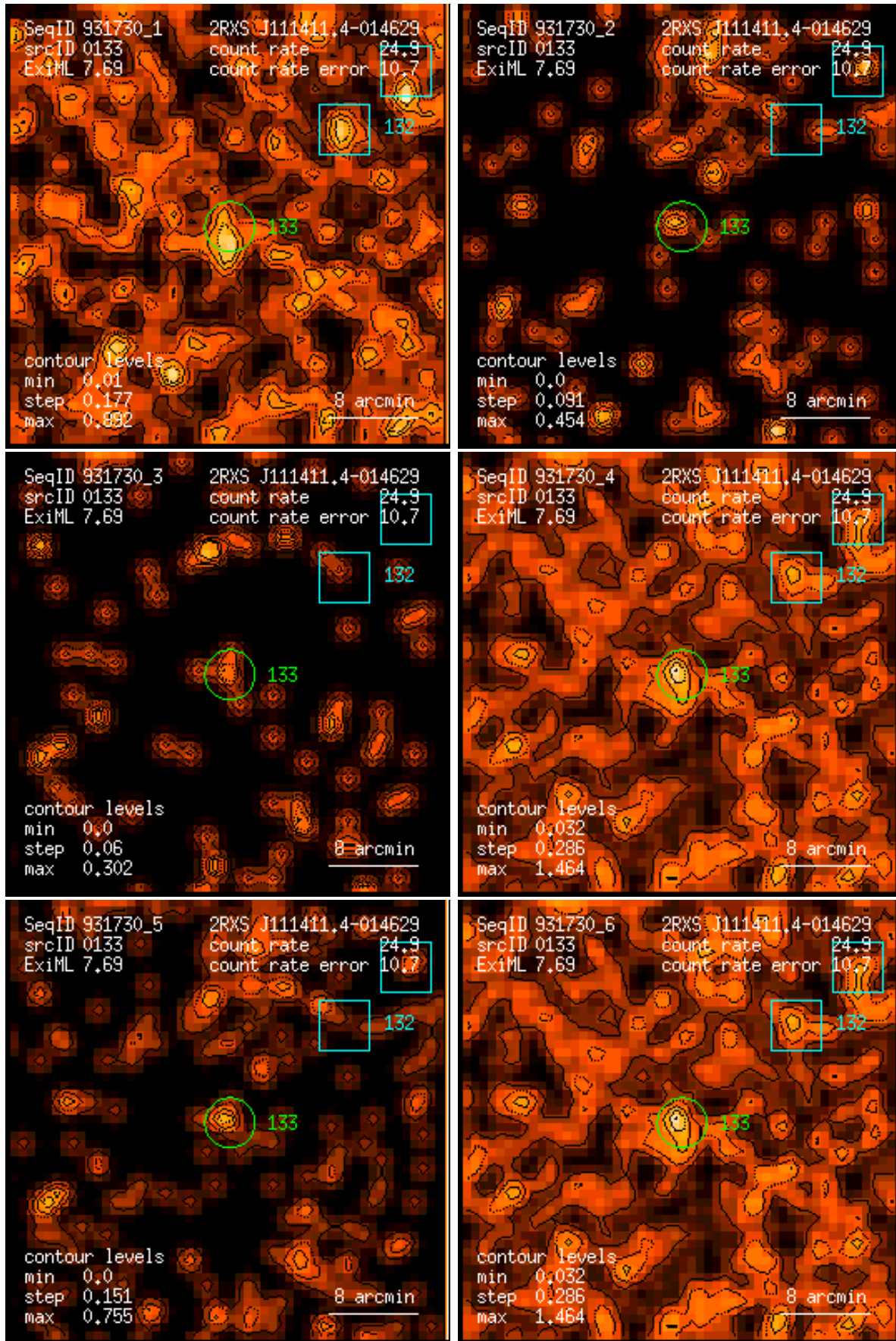
Figure 133: RASS 931730: detection 0133: band rate images, Gaussian filter: (1) PSPC channels 11 – 41, (2) 52 – 90, (3) 91 – 201, (4) 11 – 235, (5) 52 – 201, (6) 11 – 201. Broad band rates in counts/ks. Band rate contour levels in counts/ks/arcmin 2 .
