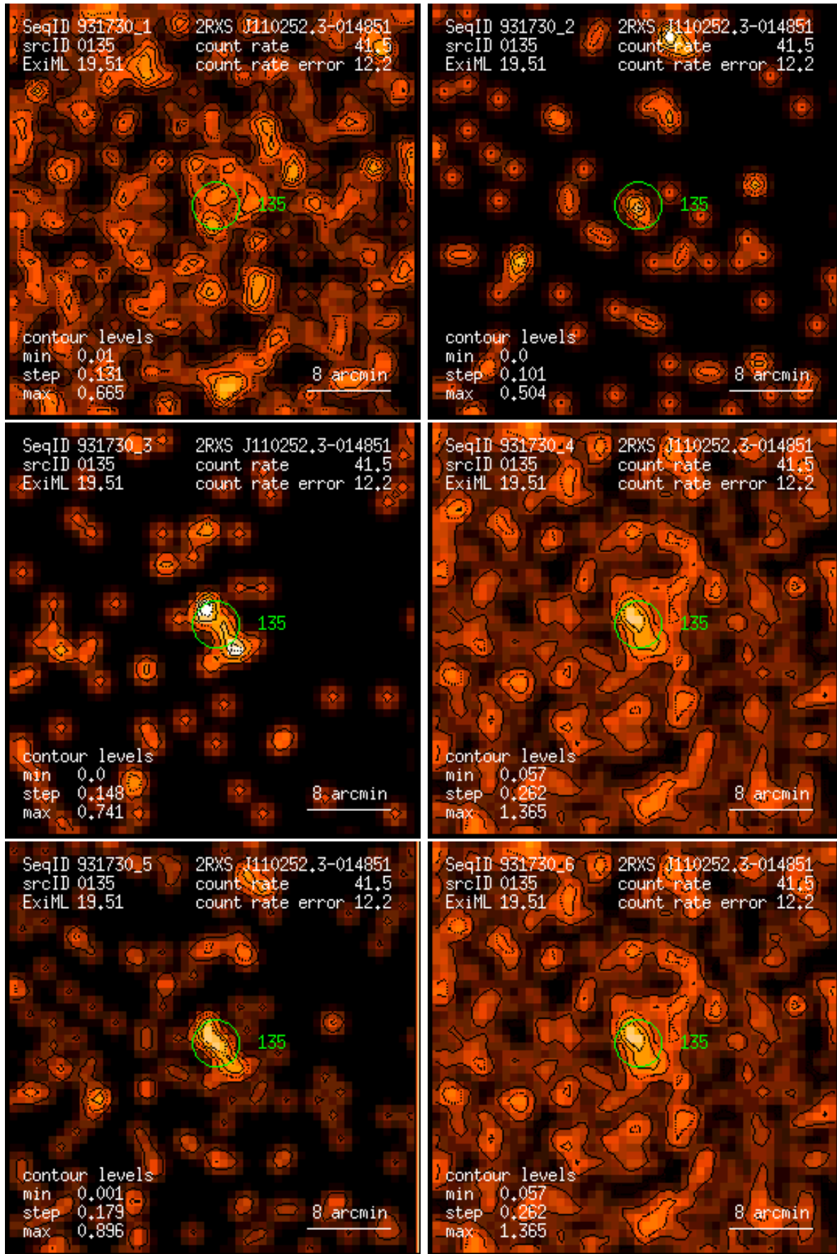
Figure 135: RASS 931730: detection 0135: band rate images, Gaussian filter: (1) PSPC channels 11 – 41, (2) 52 – 90, (3) 91 – 201, (4) 11 – 235, (5) 52 – 201, (6) 11 – 201. Broad band rates in counts/ks. Band rate contour levels in counts/ks/arcmin 2 .
