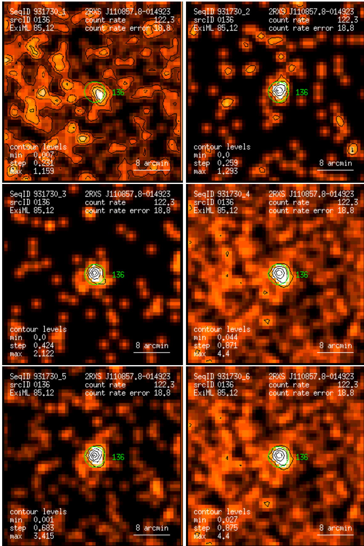
Figure 136: RASS 931730: detection 0136: band rate images, Gaussian filter: (1) PSPC channels 11 – 41, (2) 52 – 90, (3) 91 – 201, (4) 11 – 235, (5) 52 – 201, (6) 11 – 201. Broad band rates in counts/ks. Band rate contour levels in counts/ks/arcmin 2 .
