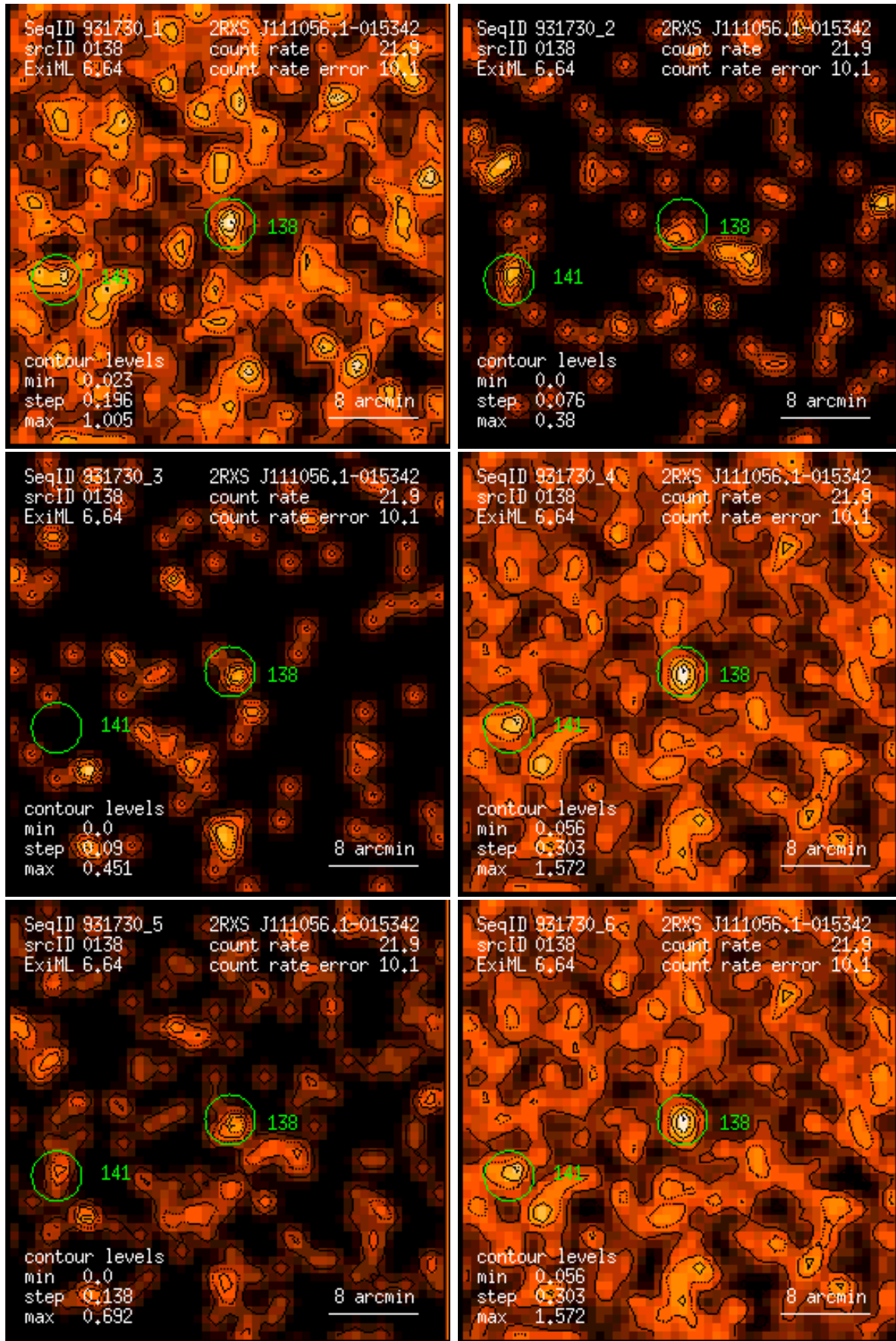
Figure 138: RASS 931730: detection 0138: band rate images, Gaussian filter: (1) PSPC channels 11 – 41, (2) 52 – 90, (3) 91 – 201, (4) 11 – 235, (5) 52 – 201, (6) 11 – 201. Broad band rates in counts/ks. Band rate contour levels in counts/ks/arcmin 2 .
