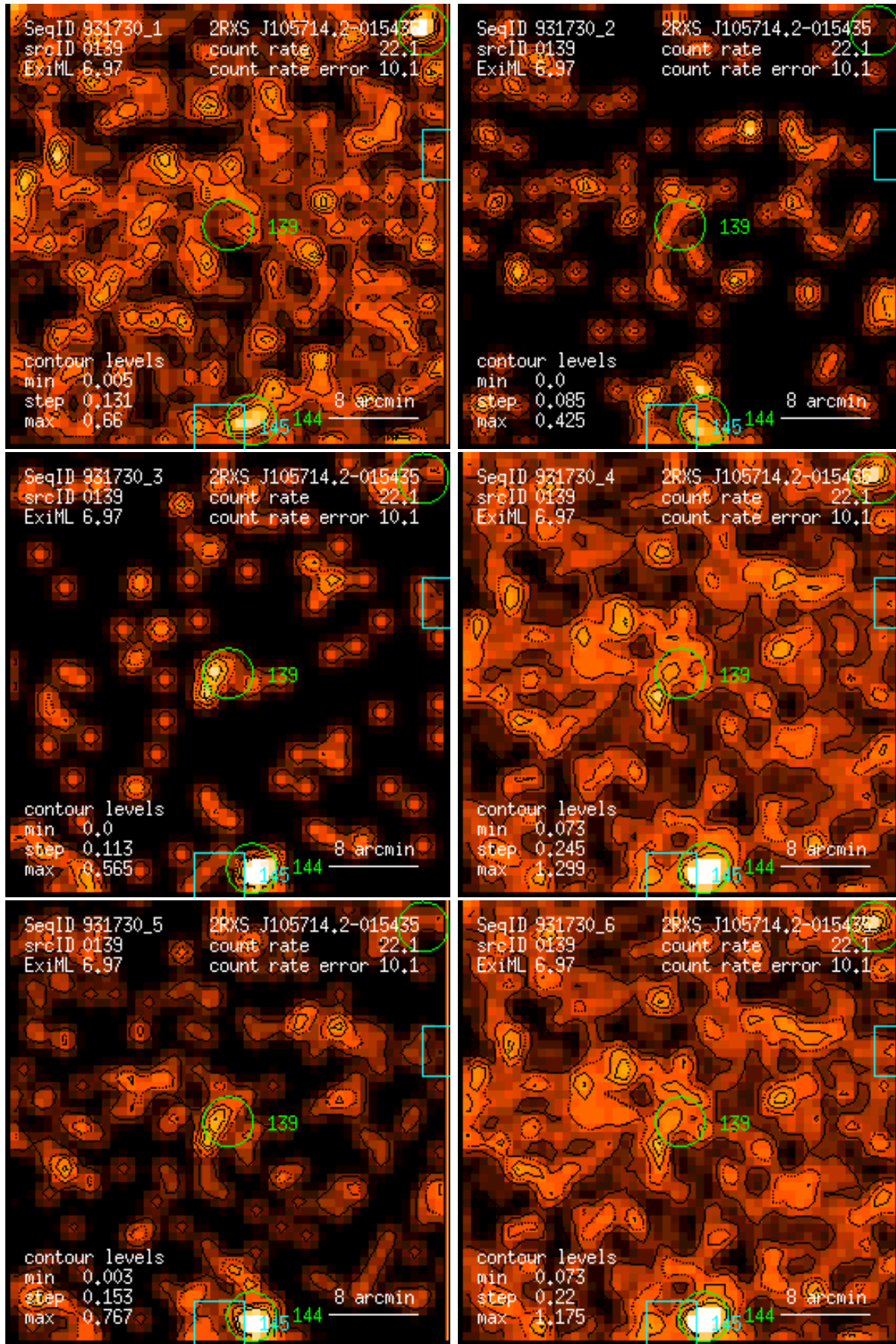
Figure 139: RASS 931730: detection 0139: band rate images, Gaussian filter: (1) PSPC channels 11 – 41, (2) 52 – 90, (3) 91 – 201, (4) 11 – 235, (5) 52 – 201, (6) 11 – 201. Broad band rates in counts/ks. Band rate contour levels in counts/ks/arcmin 2 .
