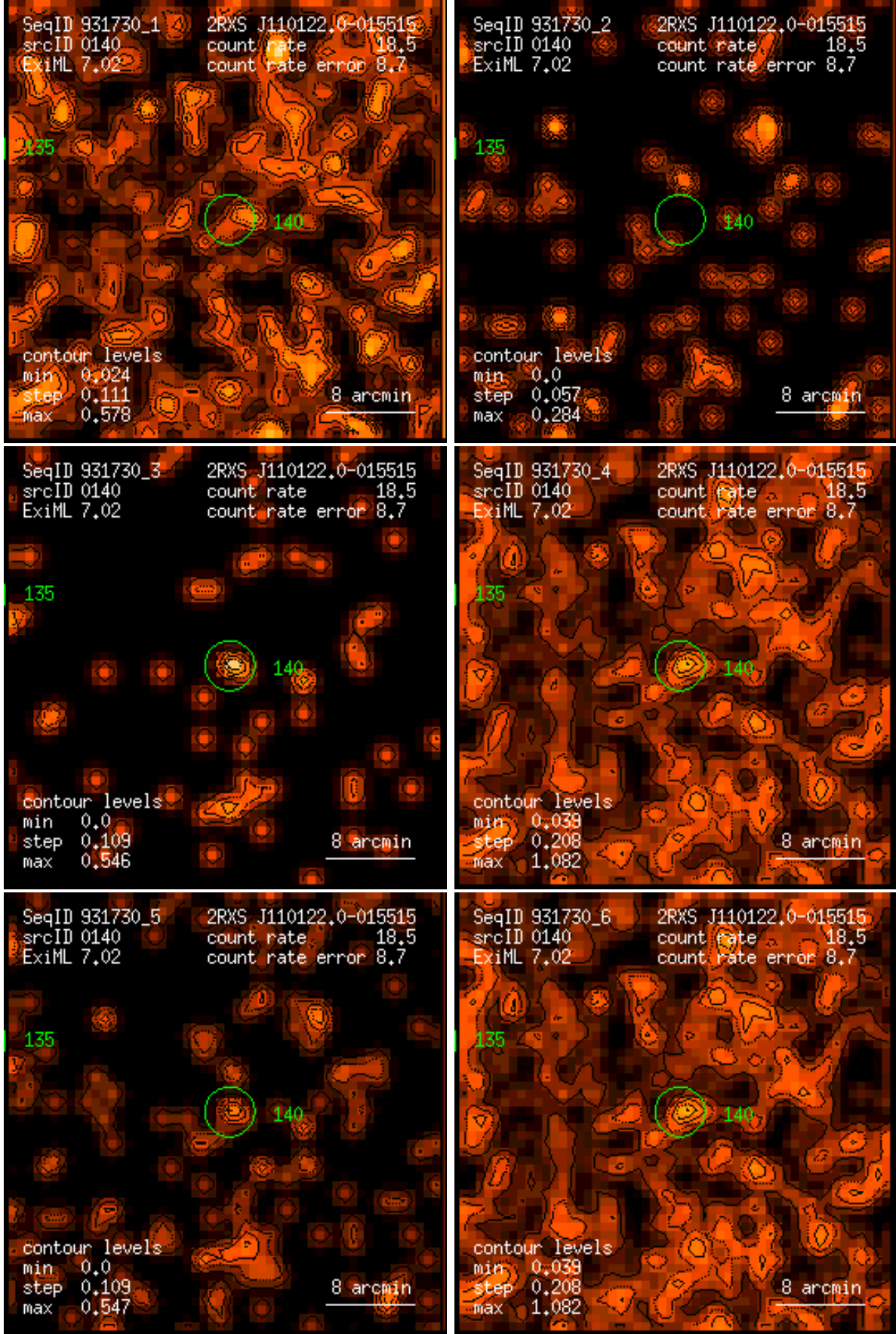
Figure 140: RASS 931730: detection 0140: band rate images, Gaussian filter: (1) PSPC channels 11 – 41, (2) 52 – 90, (3) 91 – 201, (4) 11 – 235, (5) 52 – 201, (6) 11 – 201. Broad band rates in counts/ks. Band rate contour levels in counts/ks/arcmin 2 .
